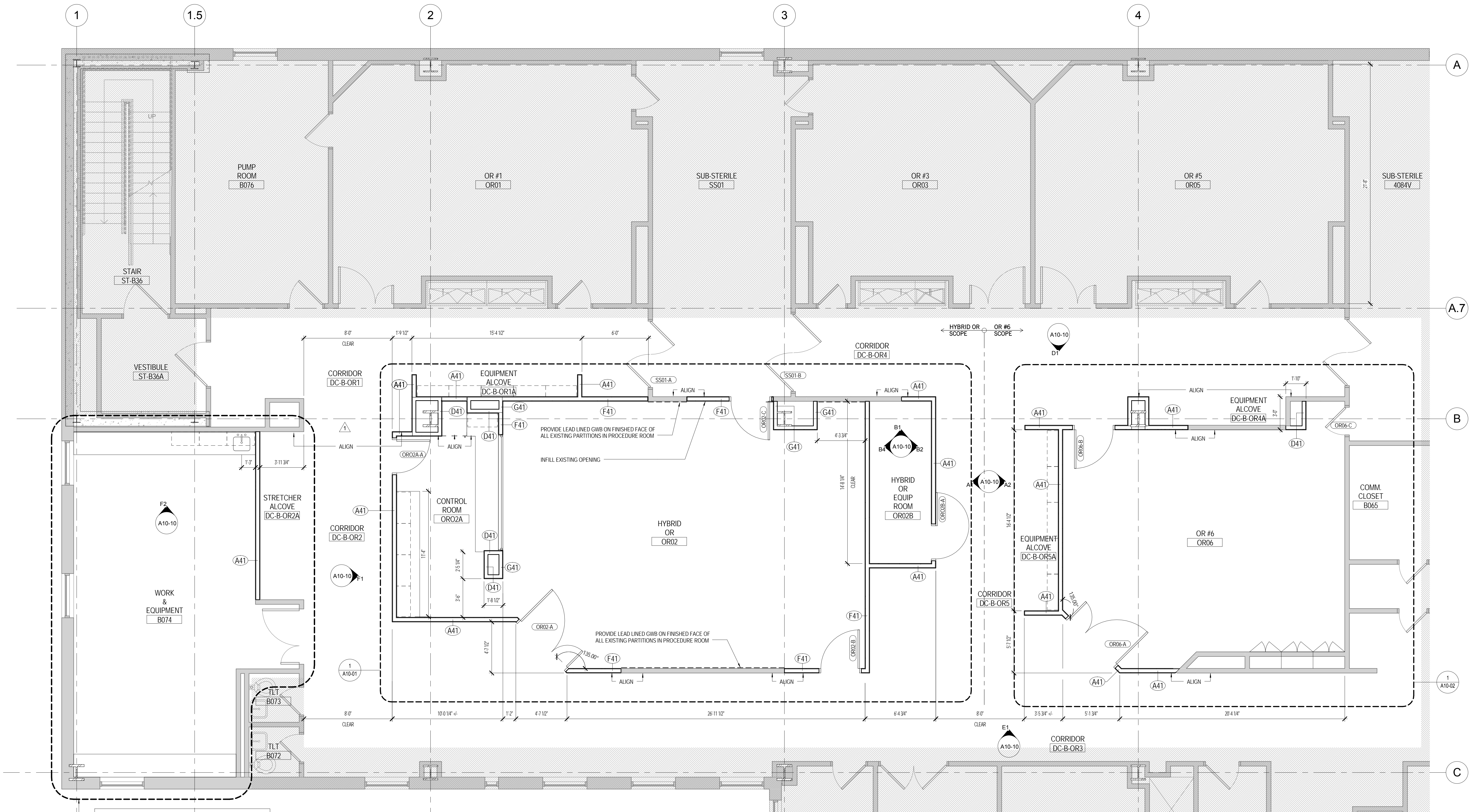
1 BASEMENT PLAN - NEW WORK 1/4" = 1'-0"
