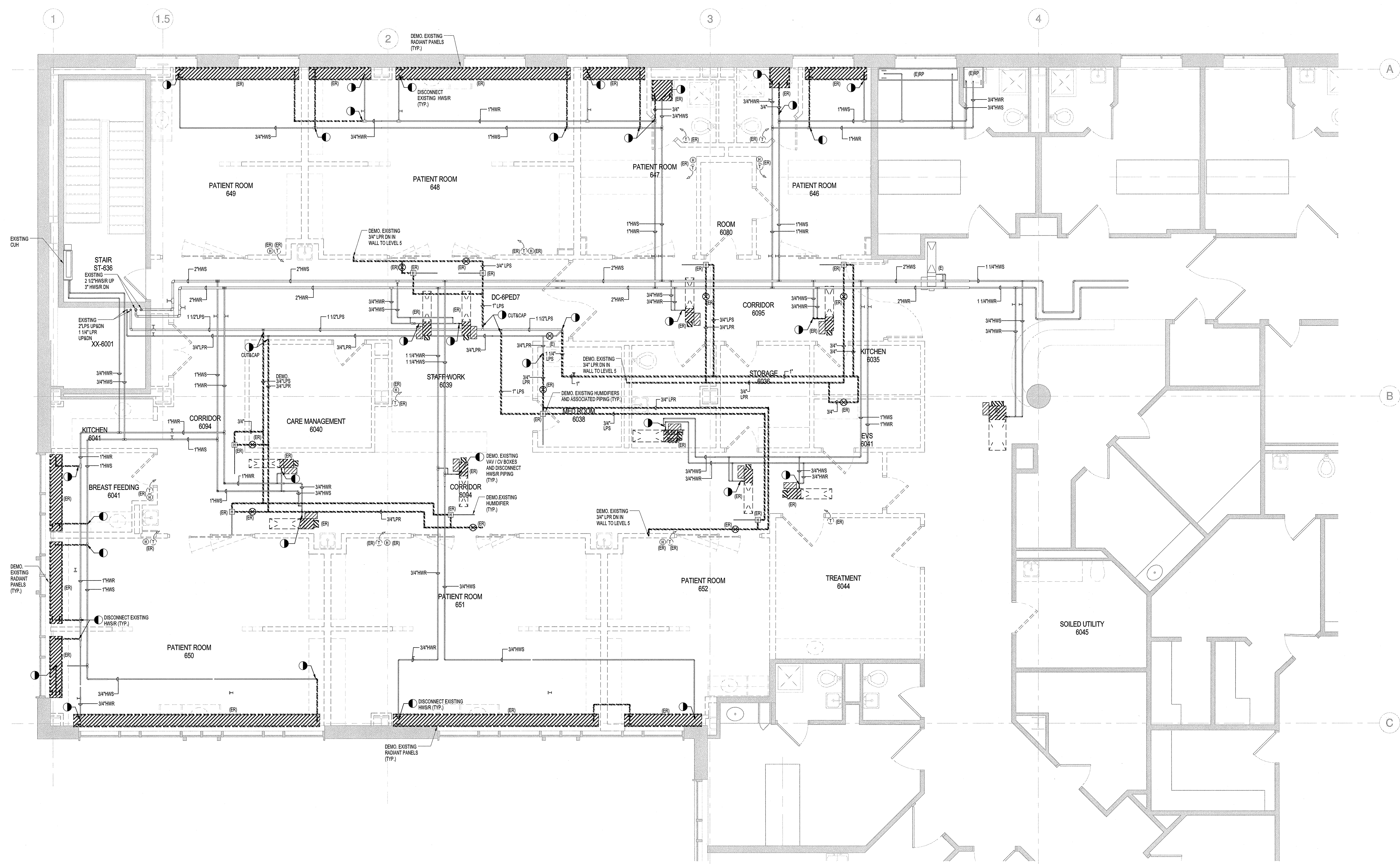
1 MECHANICAL PIPING DEMOLITION PLAN SCALE: 1/4" = 1'-0"
