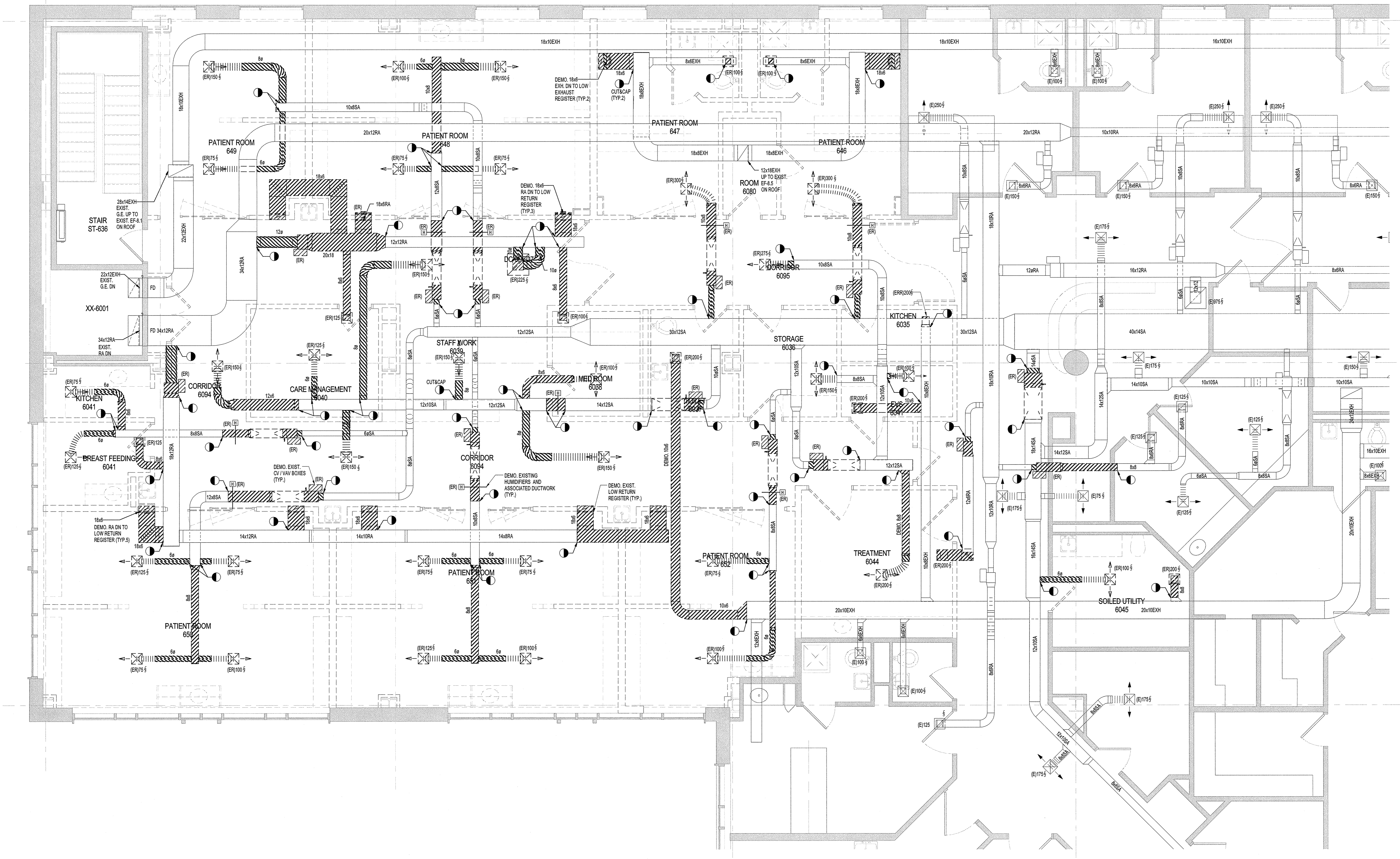
1 MECHANICAL DUCTWORK DEMOLITION PLAN SCALE: 1/4" = 1'-0"
