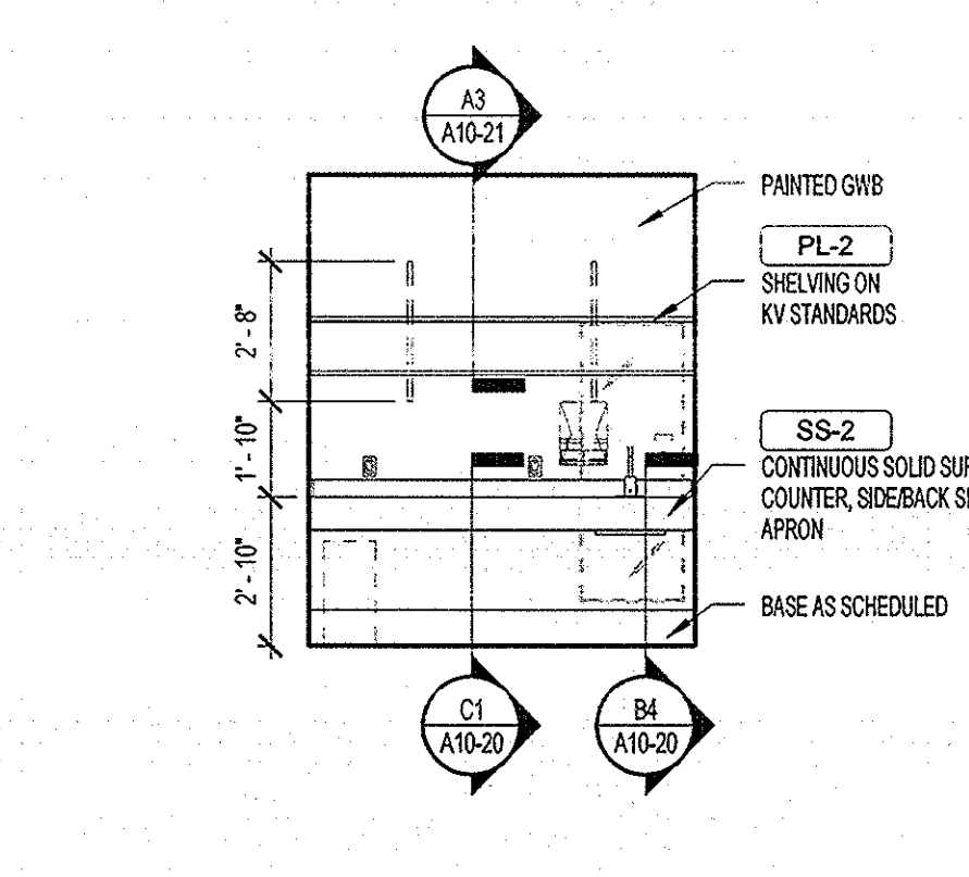
B3 SOILED - NORTH WALL 1/4" = 1'-0"
