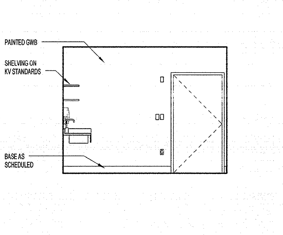
B1 SOILED - EAST WALL 1/4" = 1'-0"
