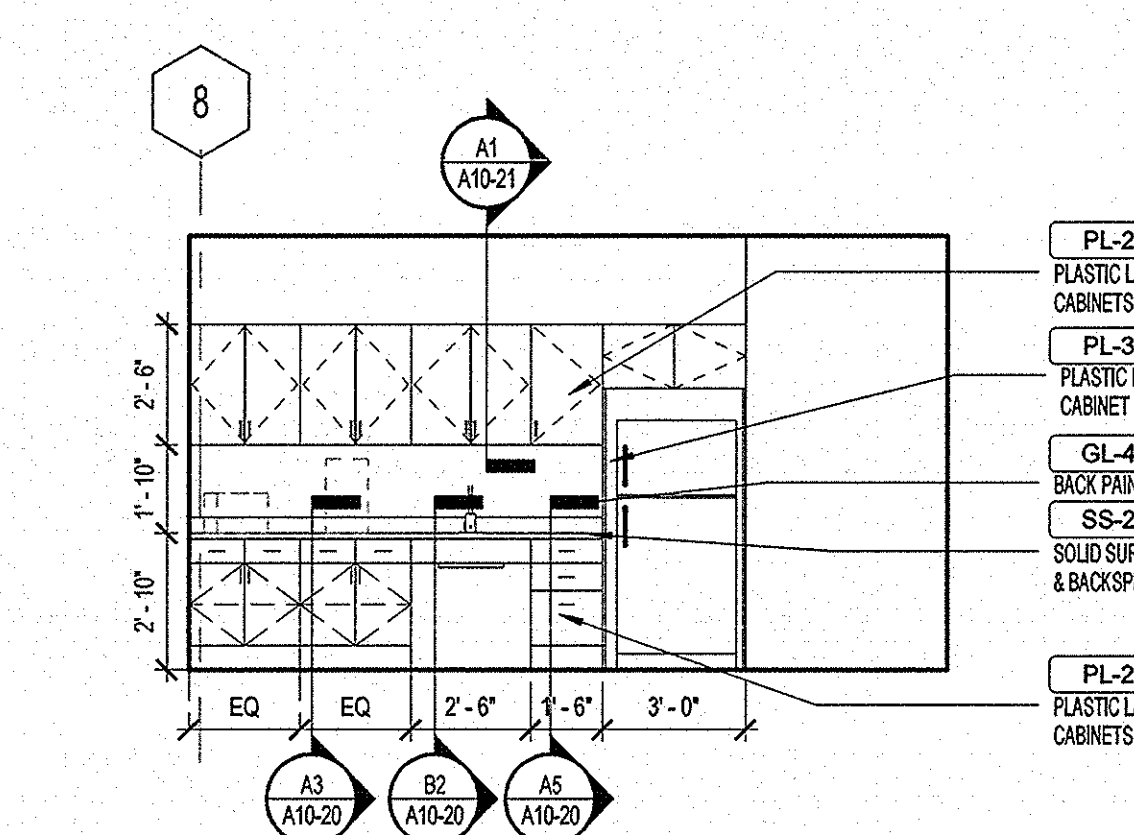
E2 STAFF LOUNGE #2025 - SOUTH 1/4" = 1'-0"
