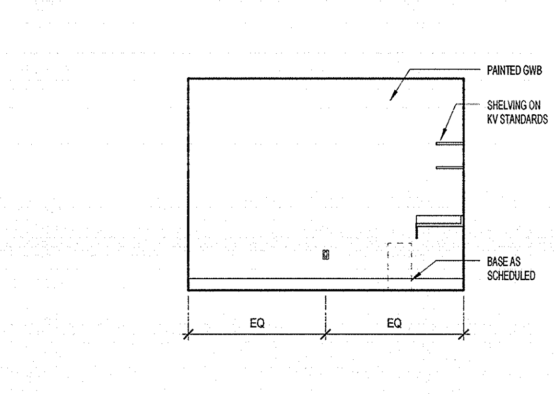
B2 SOILED - WEST WALL 1/4" = 1'-0"
