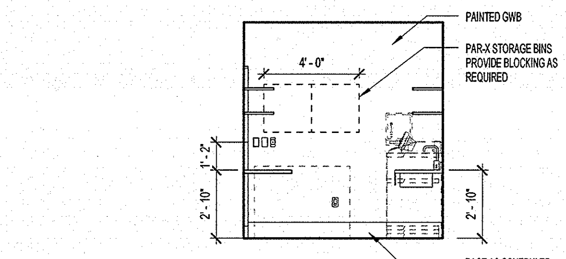
D2 MEDS - NORTH WALL 1/4" = 1'-0"
