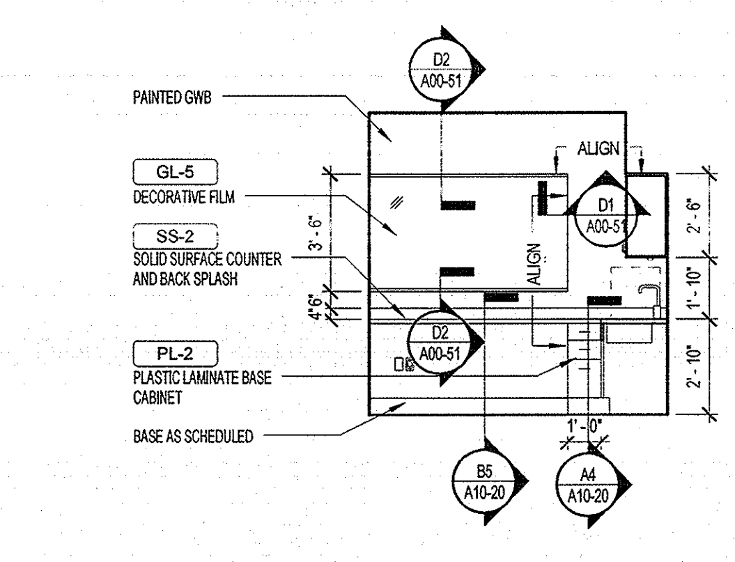
B5 STAFF LOUNGE - SOUTH 1/4" = 1'-0"
