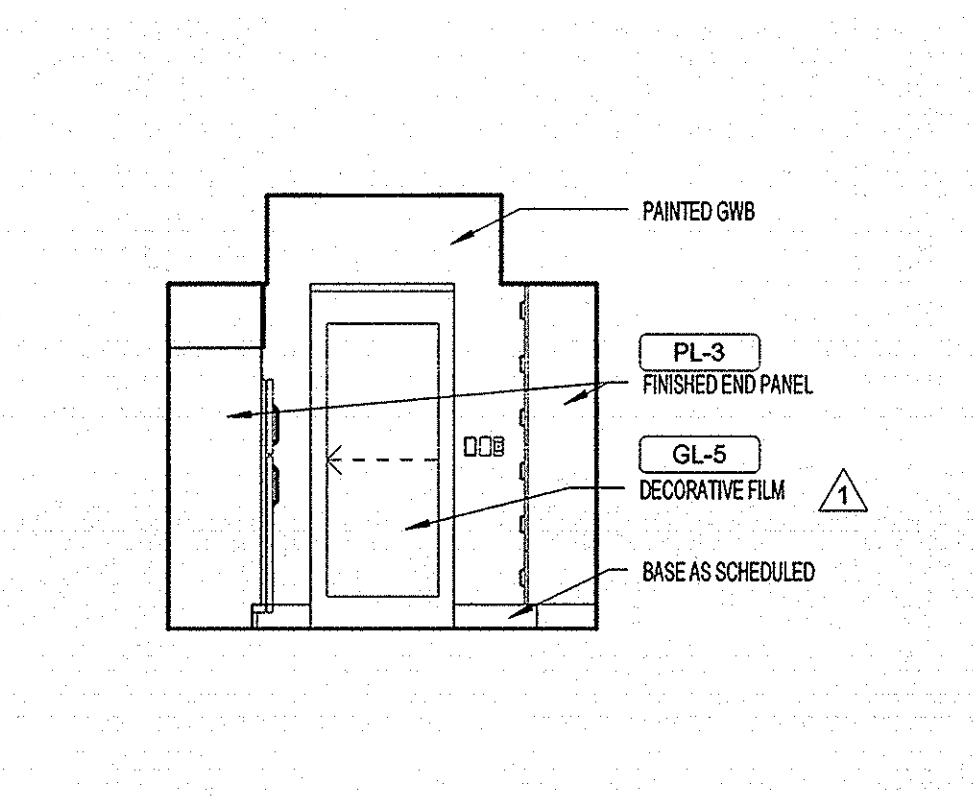
C1 STAFF LOUNGE - NORTH 1/4" = 1'-0"
