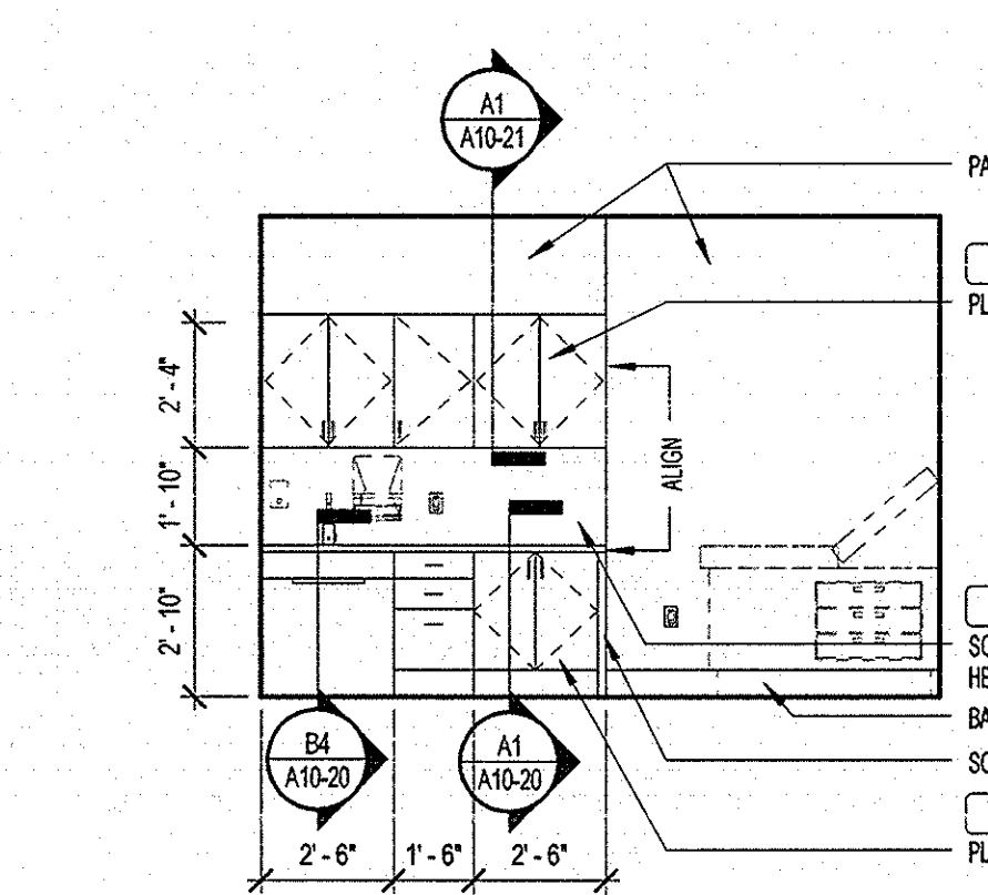
C3 TREATMENT - NORTH WALL 1/4" = 1'-0"
