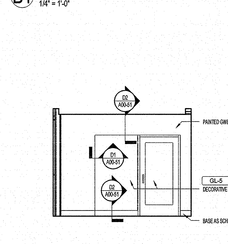
A1 CONSULTATION - ENTRY WALL 1/4" = 1'-0"
