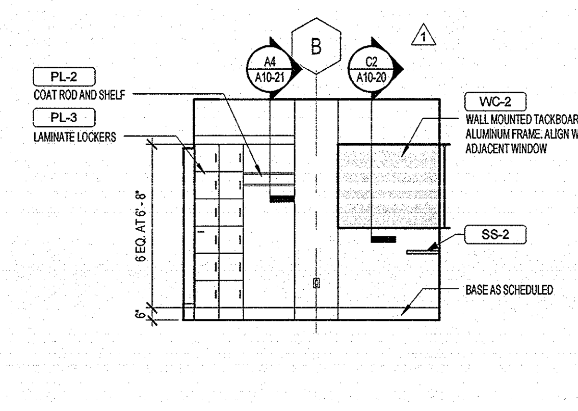
C2 STAFF LOUNGE - EAST 1/4" = 1'-0"
