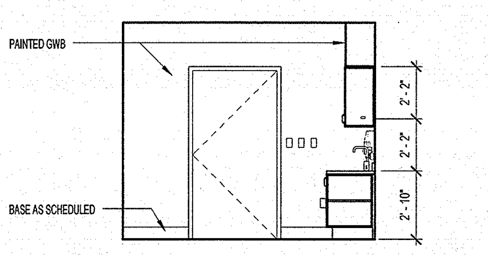
D1 TREATMENT - WEST WALL 1/4" = 1'-0"
