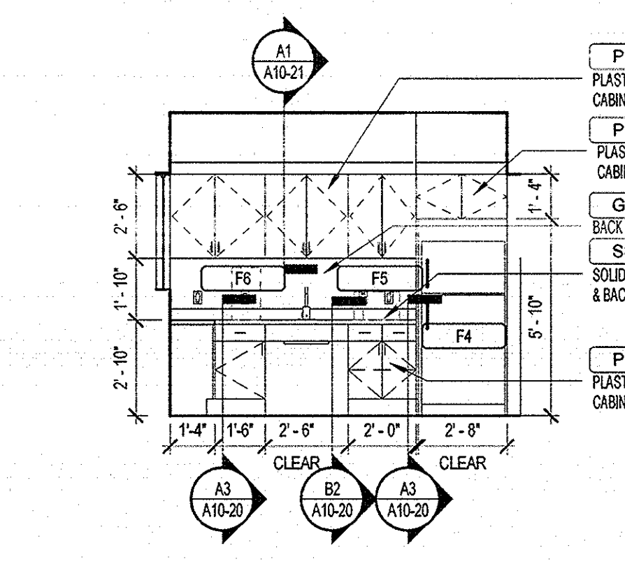
B4 STAFF LOUNGE - WEST 1/4" = 1'-0"
