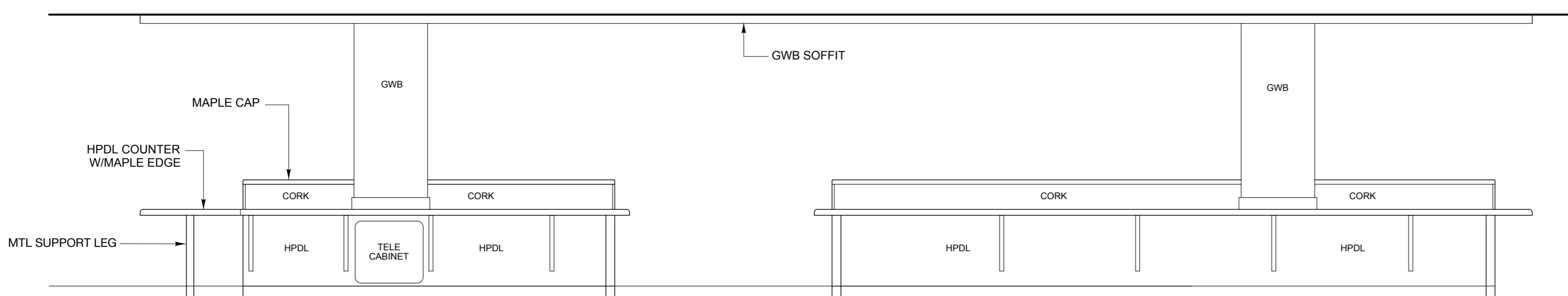
7 IMC - 6147 NURSING STATION SCALE: 3/8" = 1'-0" NORTH ELEVATION
