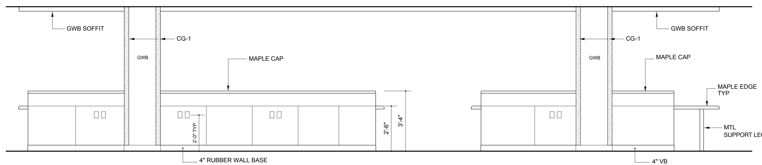
4 IMC - 6147 NURSING STATION SCALE: 3/8" = 1'-0" SOUTH ELEVATION
