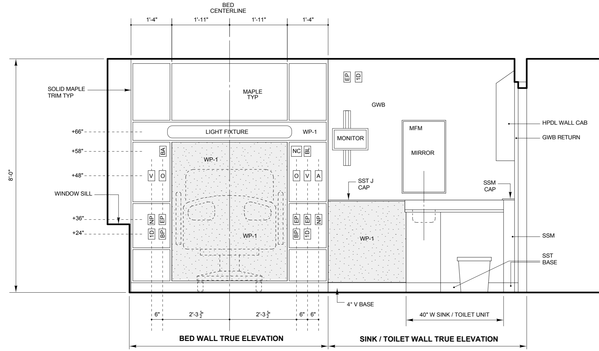
1 TYPICAL HEADWALL 1/2" = 1'-0"
