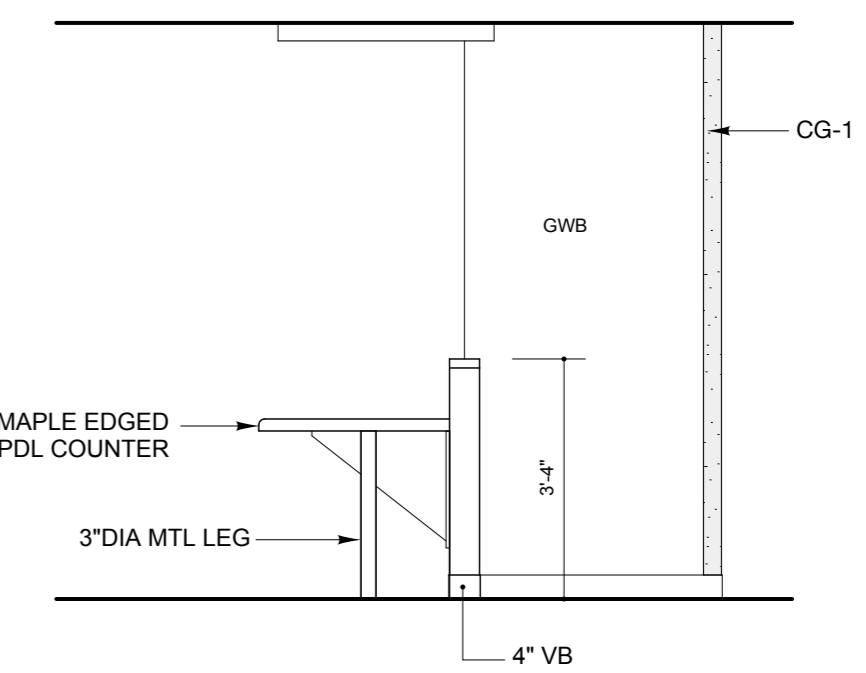
3 IMC - 6147 NURSING STATION SCALE: 3/8" = 1'-0" EAST ELEVATION
