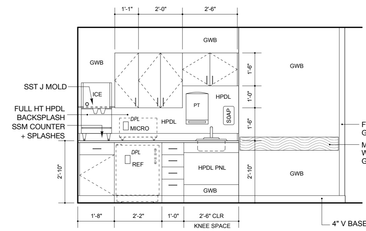
5 KITCHENETTE ROOM 6147
