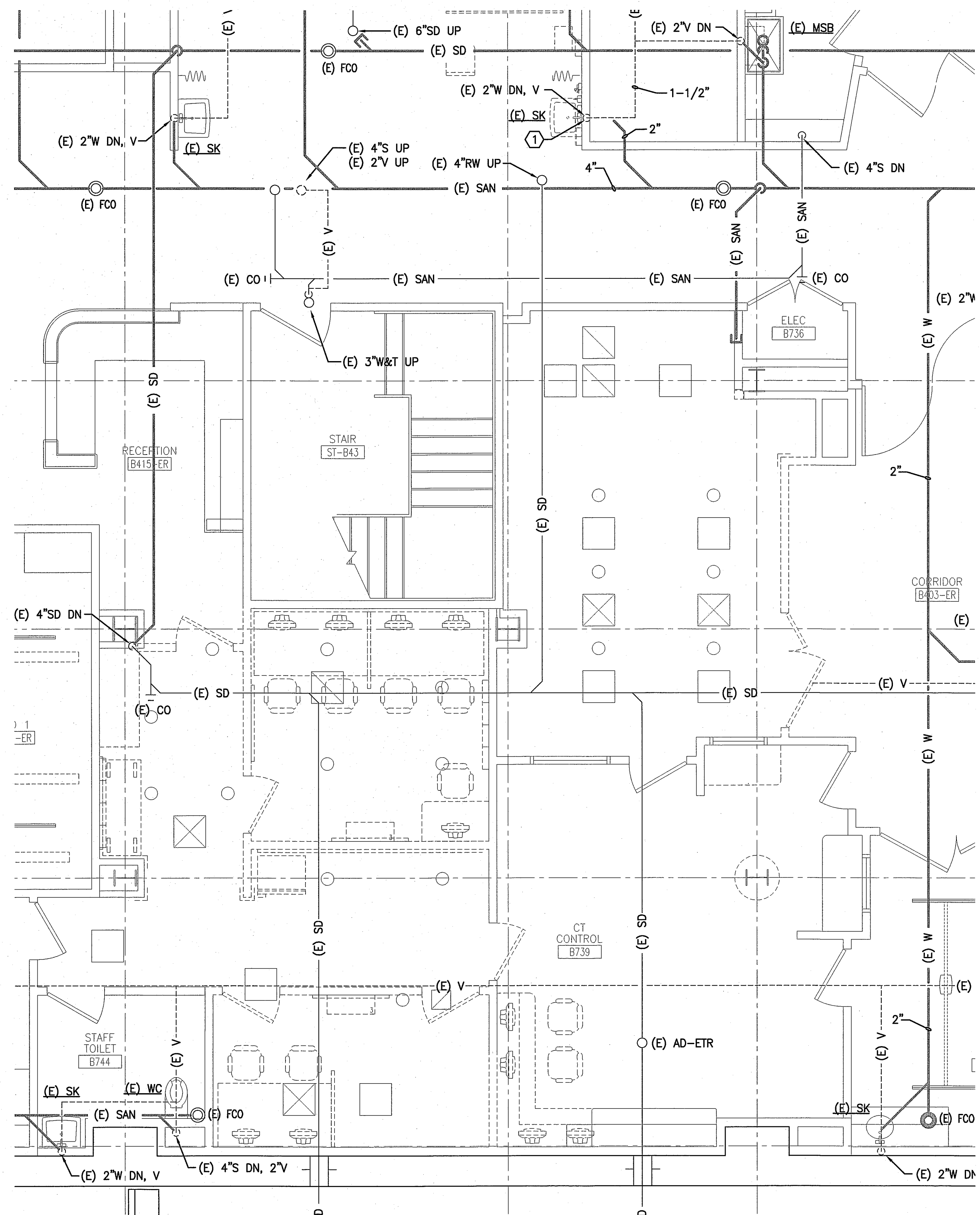
A1 DWV PIPING DEMOLITION PLAN
