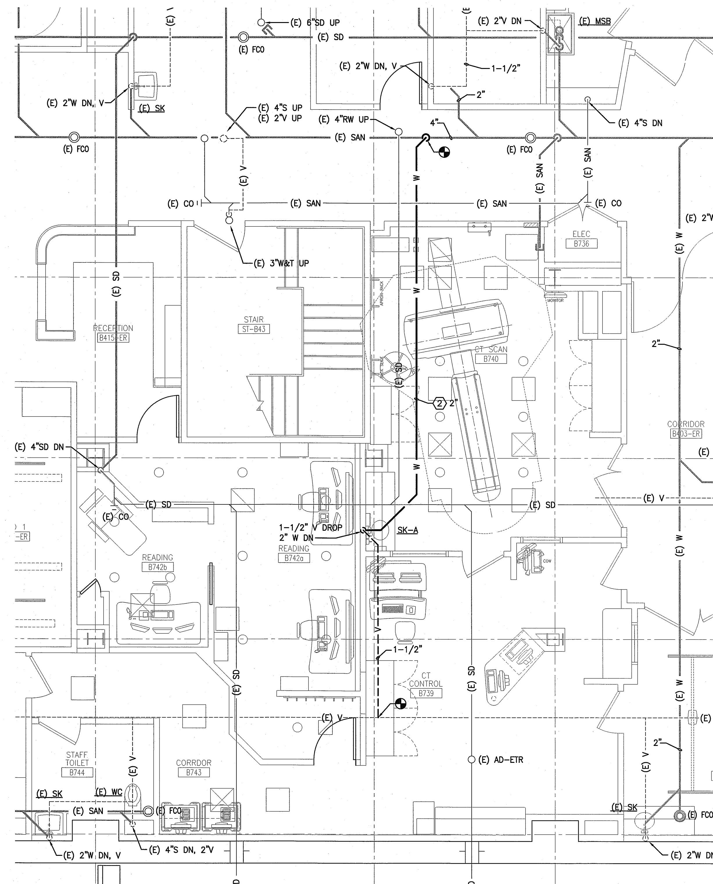
A8 DWV PIPING PLAN
