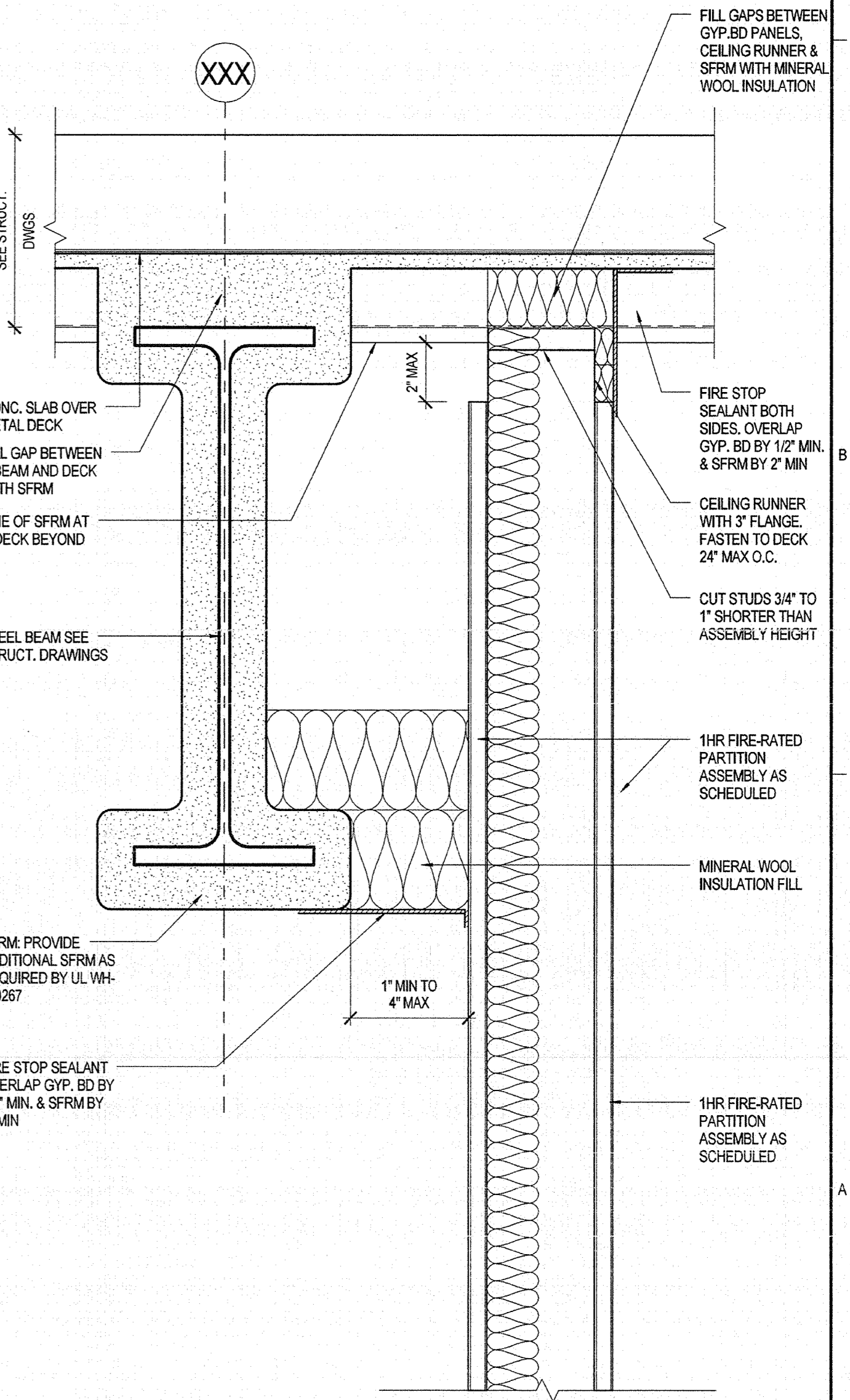
C1 PARTITION HEAD DETAIL 3" = 1'-0" 1 HR FIRE-RATED ASSEMBLY UL DESIGN HW-D-0267
