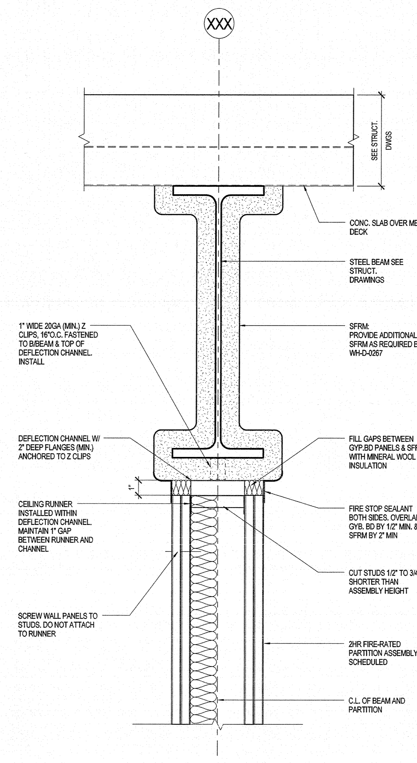
C2 PARTITION HEAD DETAIL 3" = 1'-0" 2 HR FIRE-RATED ASSEMBLY UL DESIGN HW-D-0267
