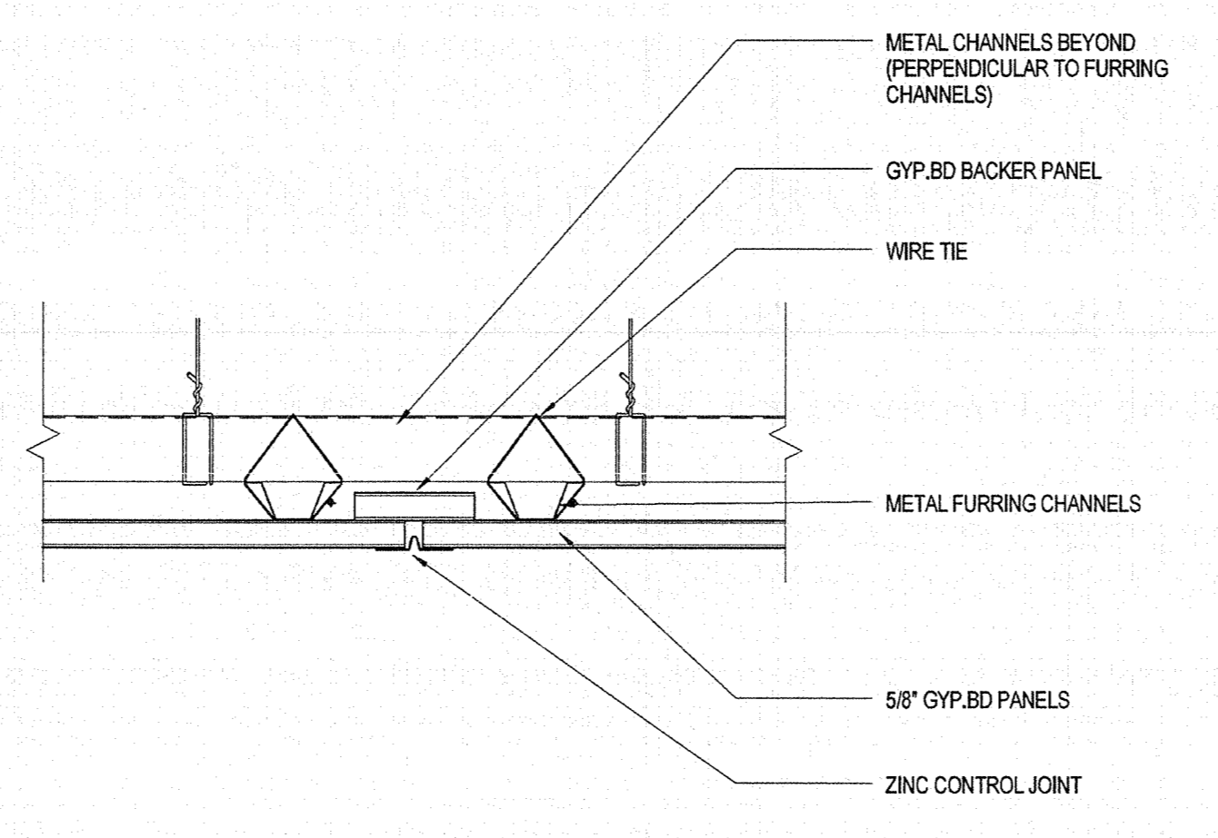
C4 CONTROL JOINT DETAIL STL. FRAMED GYP. BD CEILING 3" = 1'-0"
