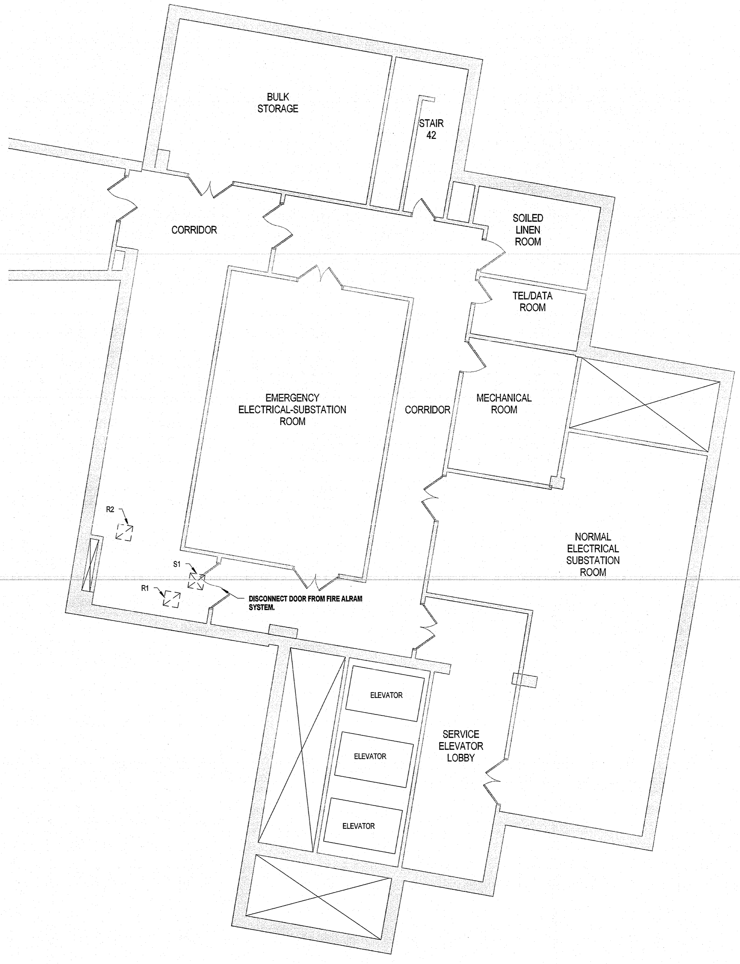
1 DEMOLITION PLAN - EAST TOWER 1/8" = 1'-0"
