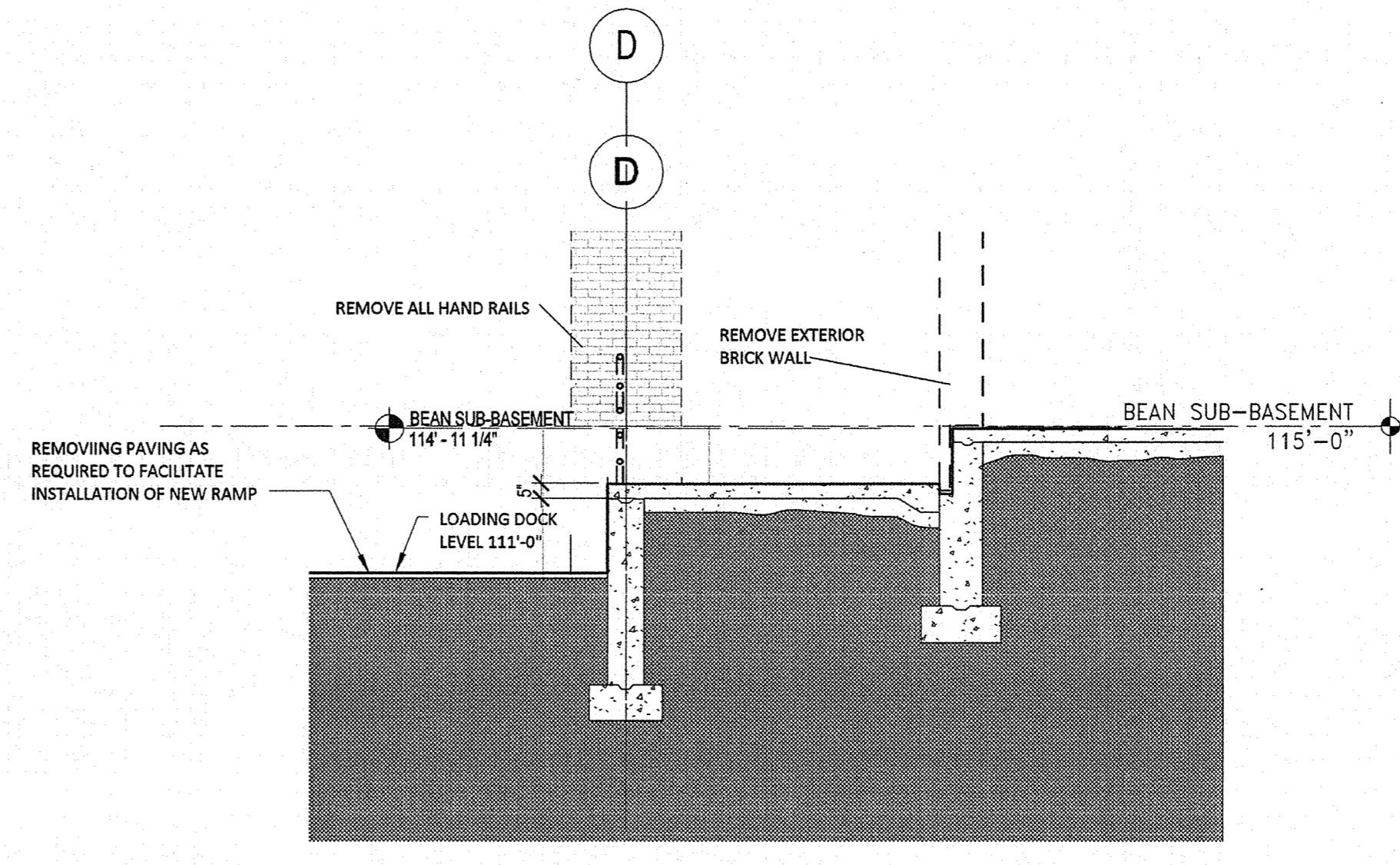
SECTION THRU EXISTING RAMP - DEMOLITION
