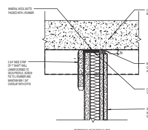
3 PARTITION HEAD DETAIL 3" x 1'-0"
