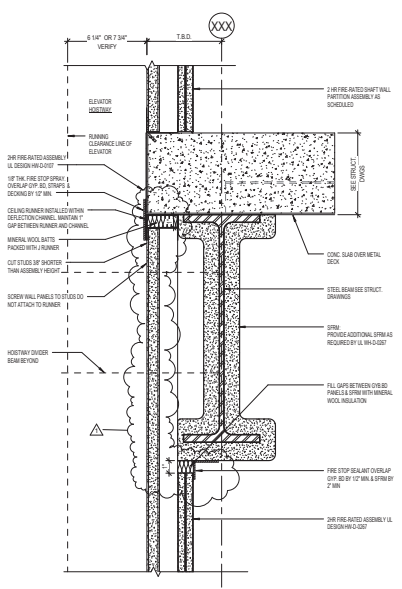
8 PARTITION HEAD DETAIL 3" x 1'-0"
