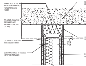
1 PARTITION HEAD DETAIL 3" x 1'-0"
