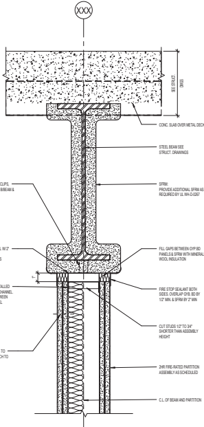
5 PARTITION HEAD DETAIL 3" x 1'-0"
