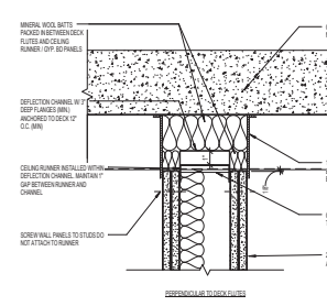
4 PARTITION HEAD DETAIL 3" x 1'-0"
