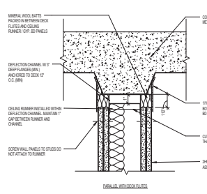
2 PARTITION HEAD DETAIL 3" x 1'-0"
