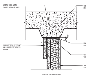
1 PARTITION HEAD DETAIL 3" x 1'-0"
