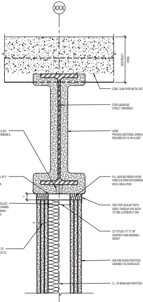
6 PARTITION HEAD DETAIL 3" x 1'-0"
