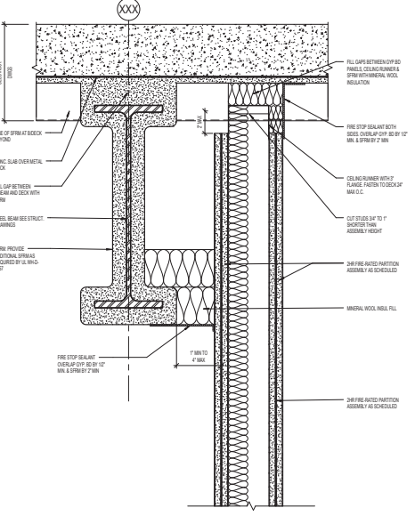
7 PARTITION HEAD DETAIL 3" x 1'-0"
