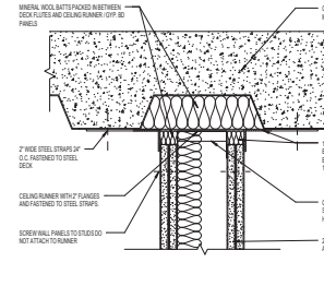
2 PARTITION HEAD DETAIL 3" x 1'-0"
