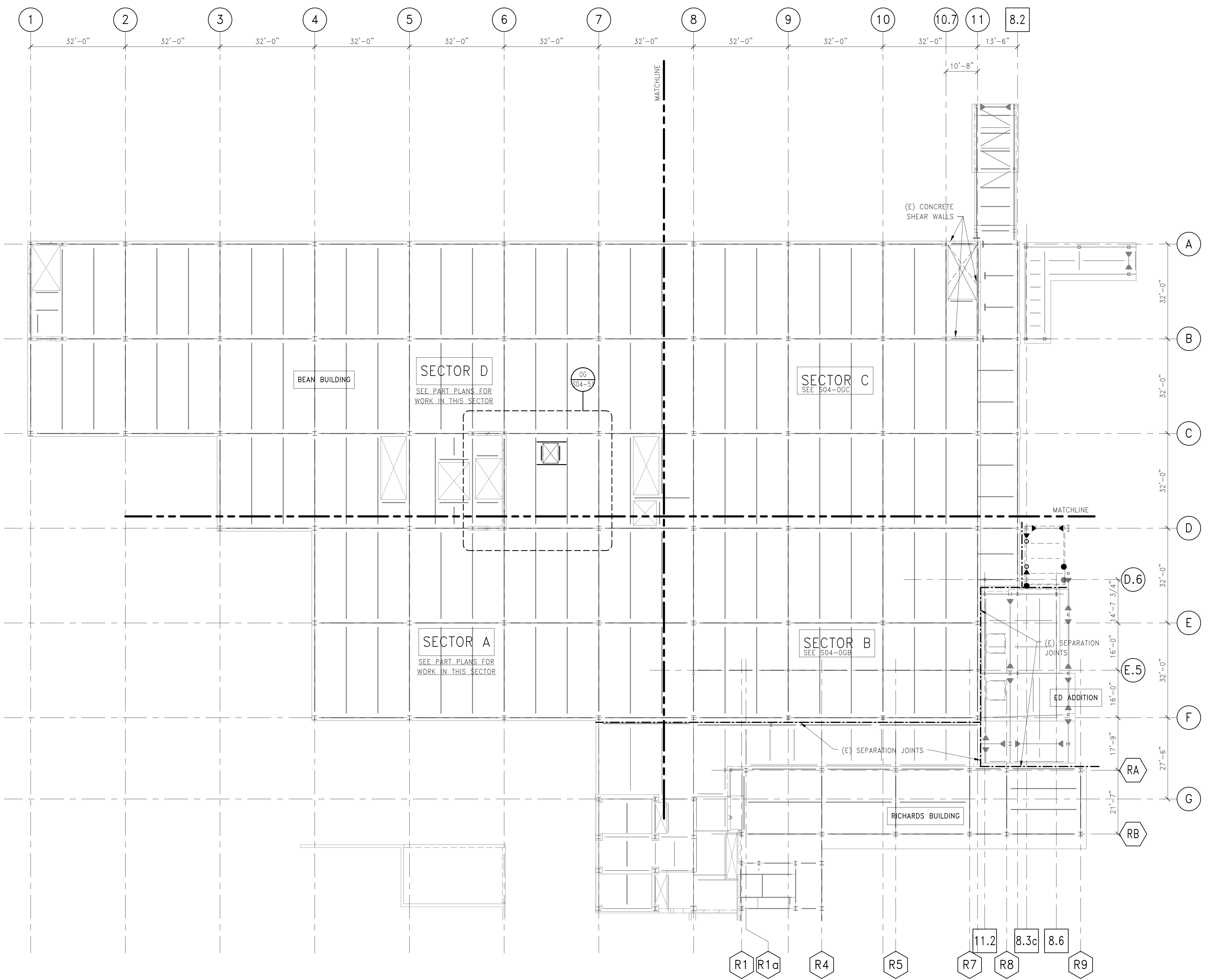
GROUND FLOOR FRAMING PLAN 1/16" = 1'-0"
