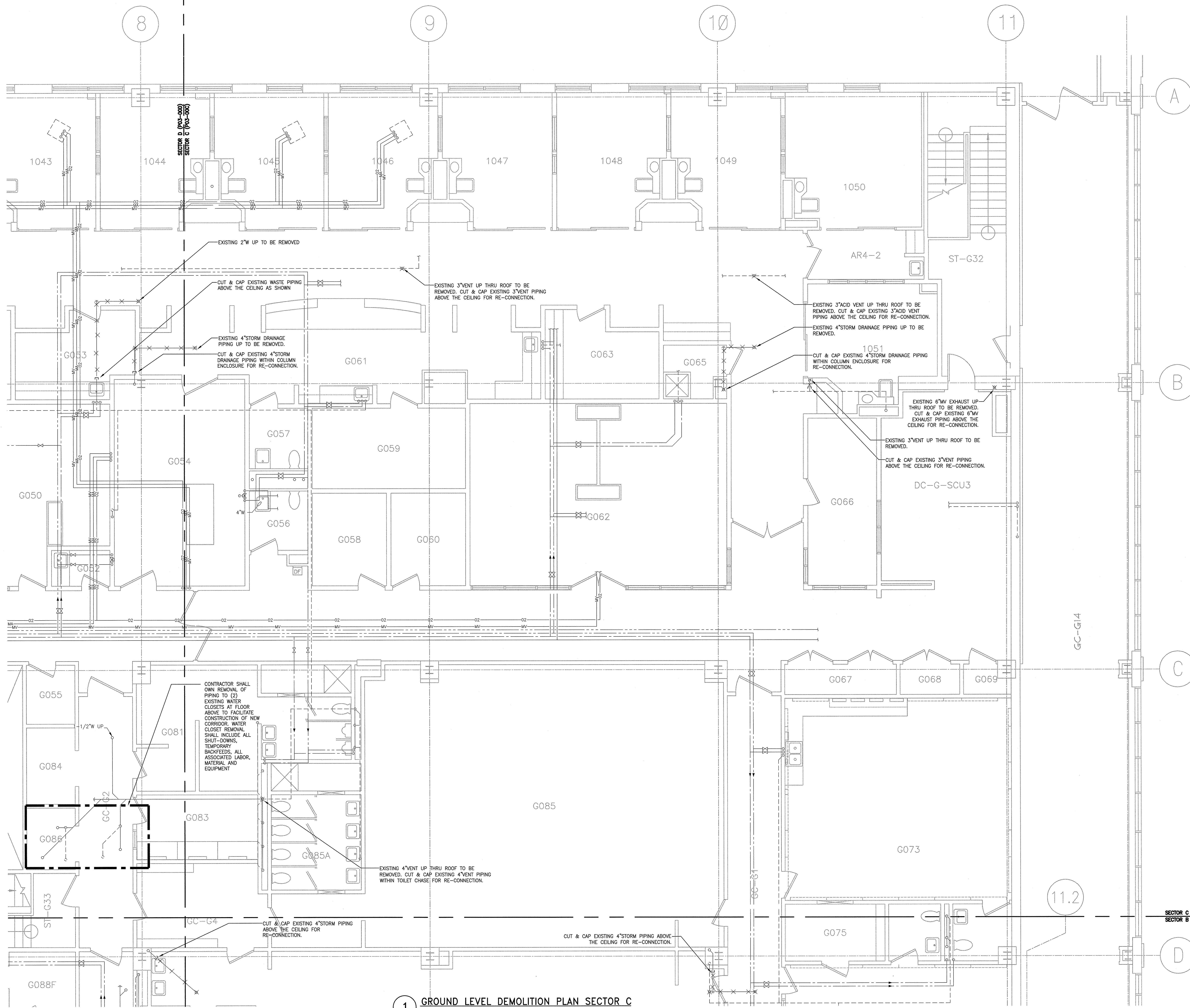
1 GROUND LEVEL DEMOLITION PLAN SECTOR C SCALE: 1/4"=1'-0"
