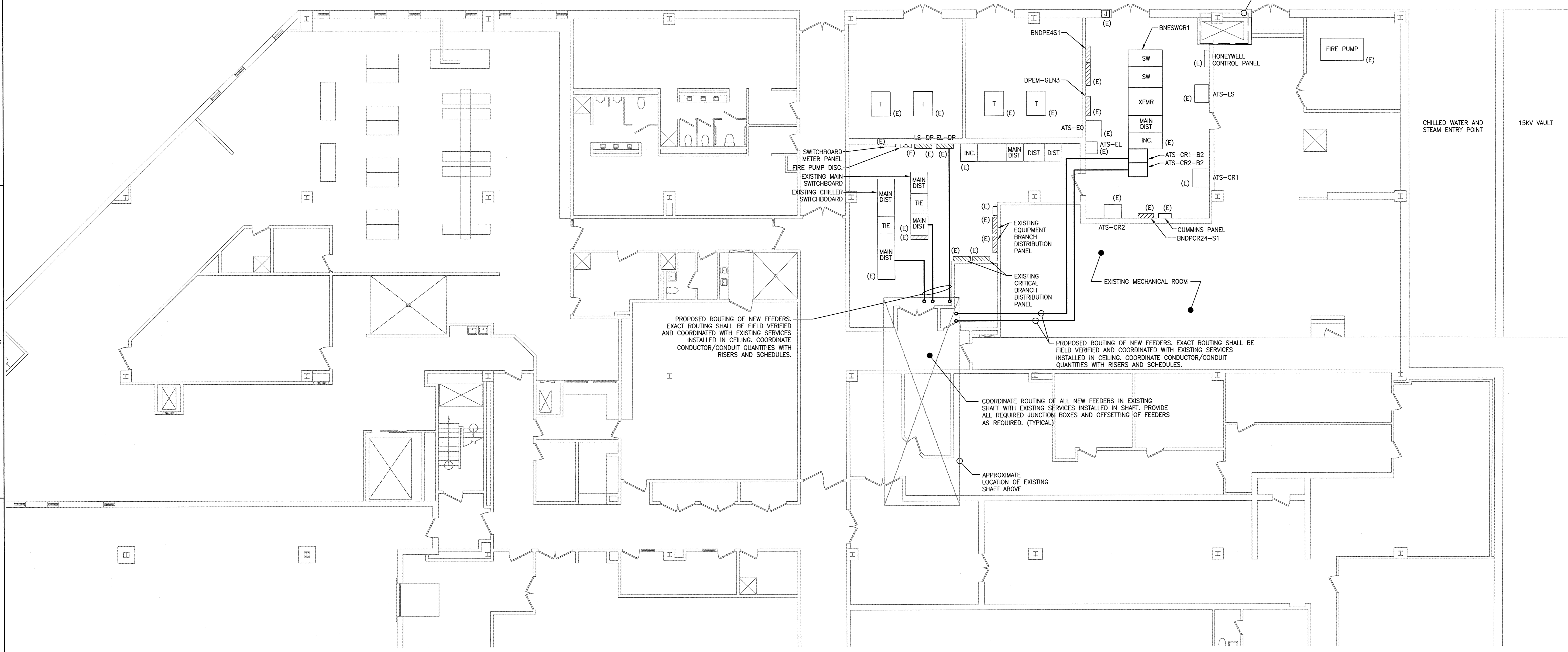
1 ELECTRICAL SUB-BASEMENT POWER PLAN - ELECTRIC ROOMS SCALE: 1/8" = 1'-0"
