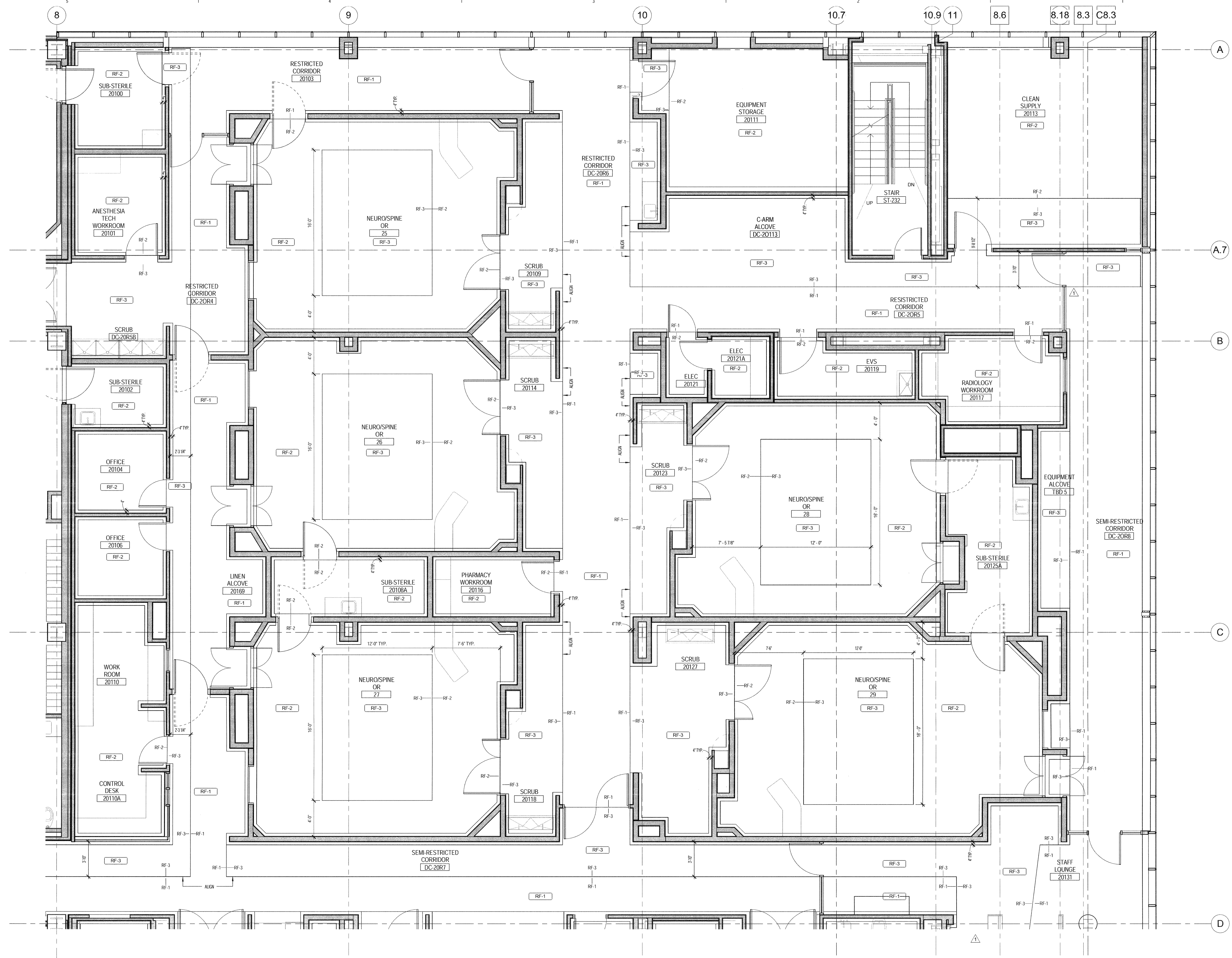
LEVEL 02 ENLARGED FLOOR PATTERN PLAN - SECTOR C A1 1/4" = 1'-0"
