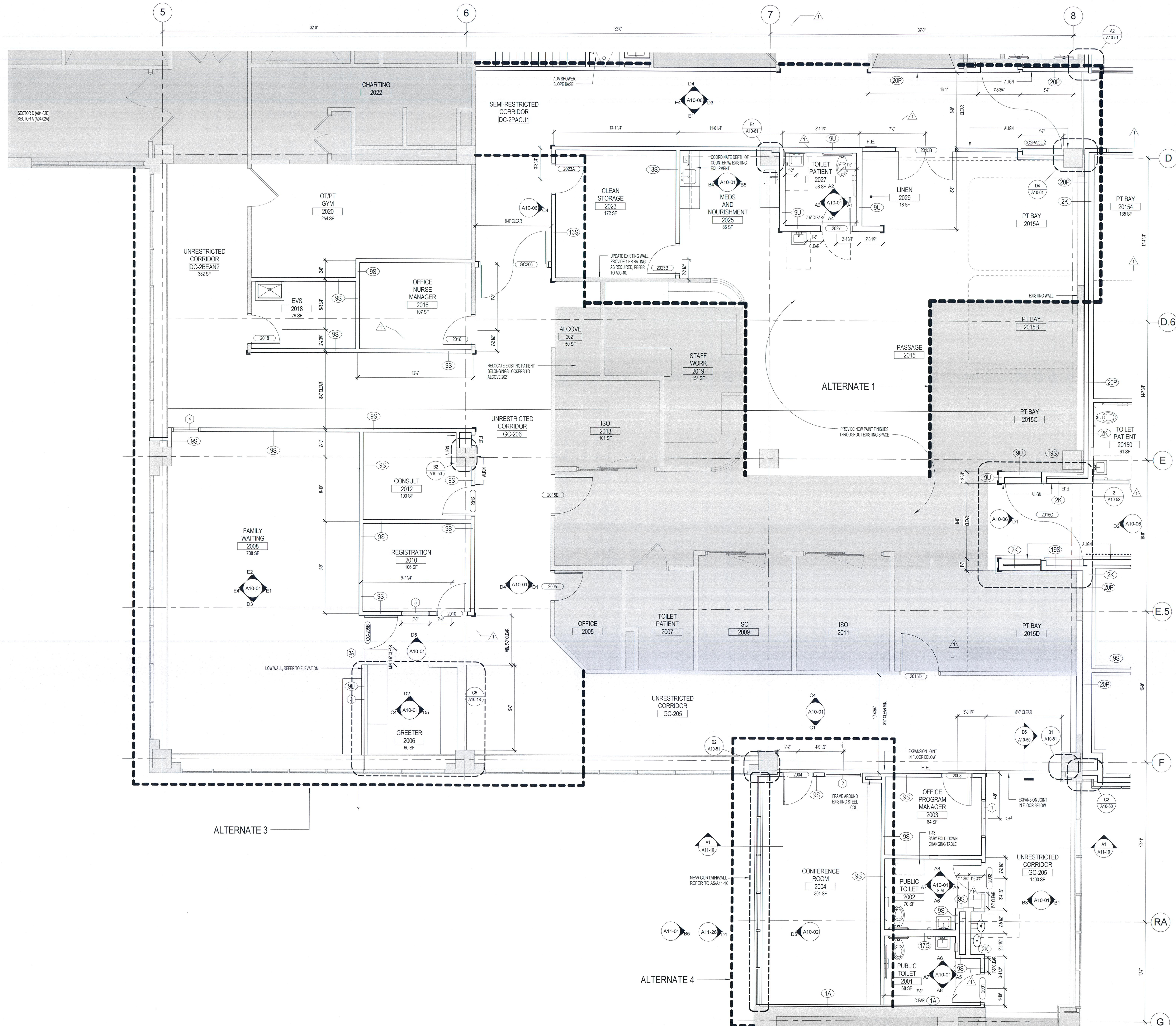
A2 LEVEL 2 FLOOR PLAN - SECTOR A 1/4" = 1'-0"
