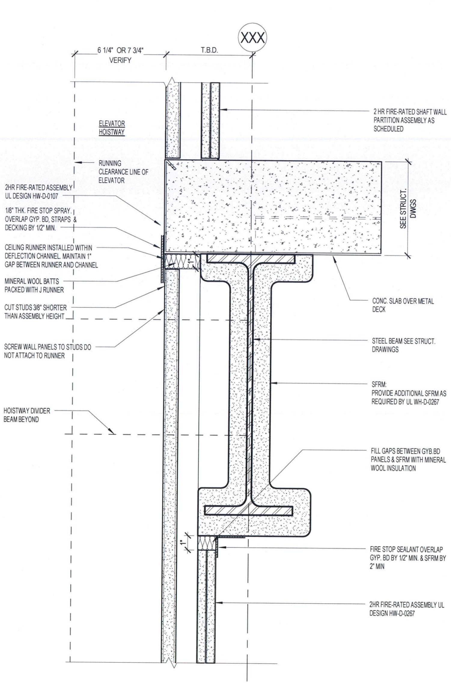
8 PARTITION HEAD DETAIL 3" = 1'-0" 2 HR FIRE-RATED ASSEMBLY UL DESIGN HW-D-0107 - HW-D-0267
