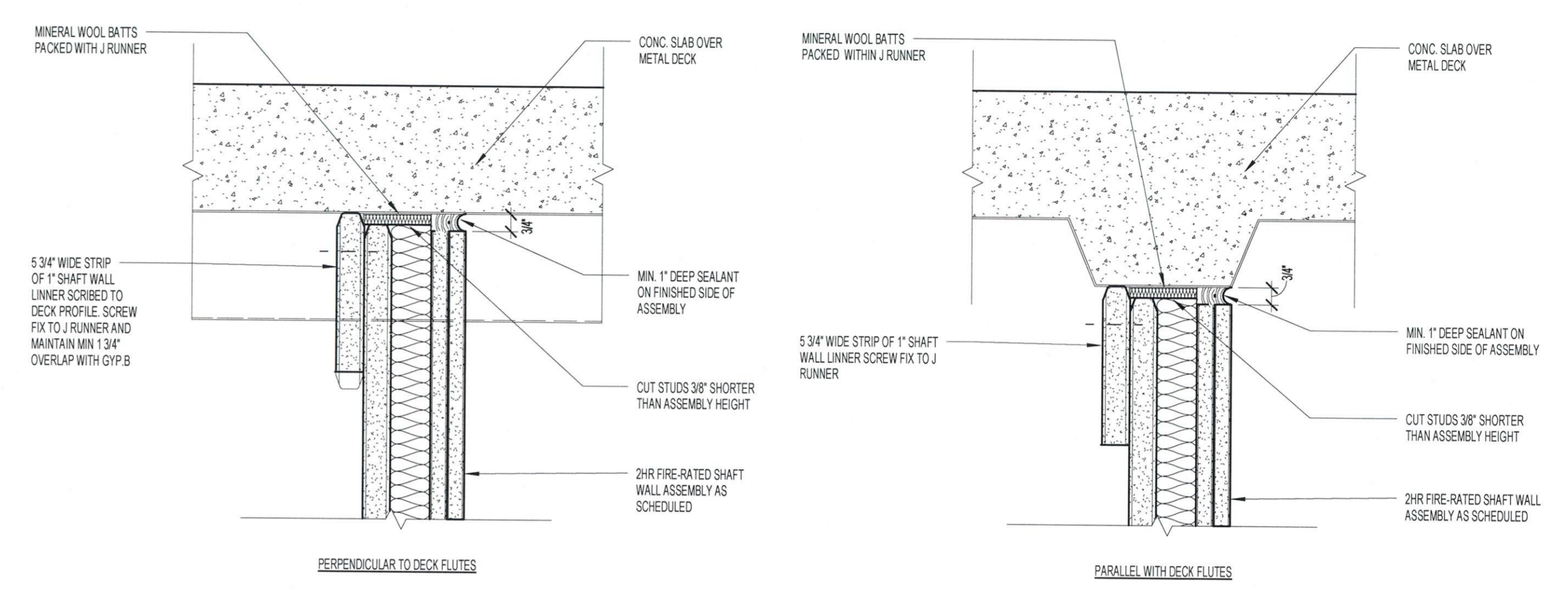
3 PARTITION HEAD DETAIL 3" = 1'-0" 2 HR FIRE-RATED ASSEMBLY UL DESIGN HW-D-0372
