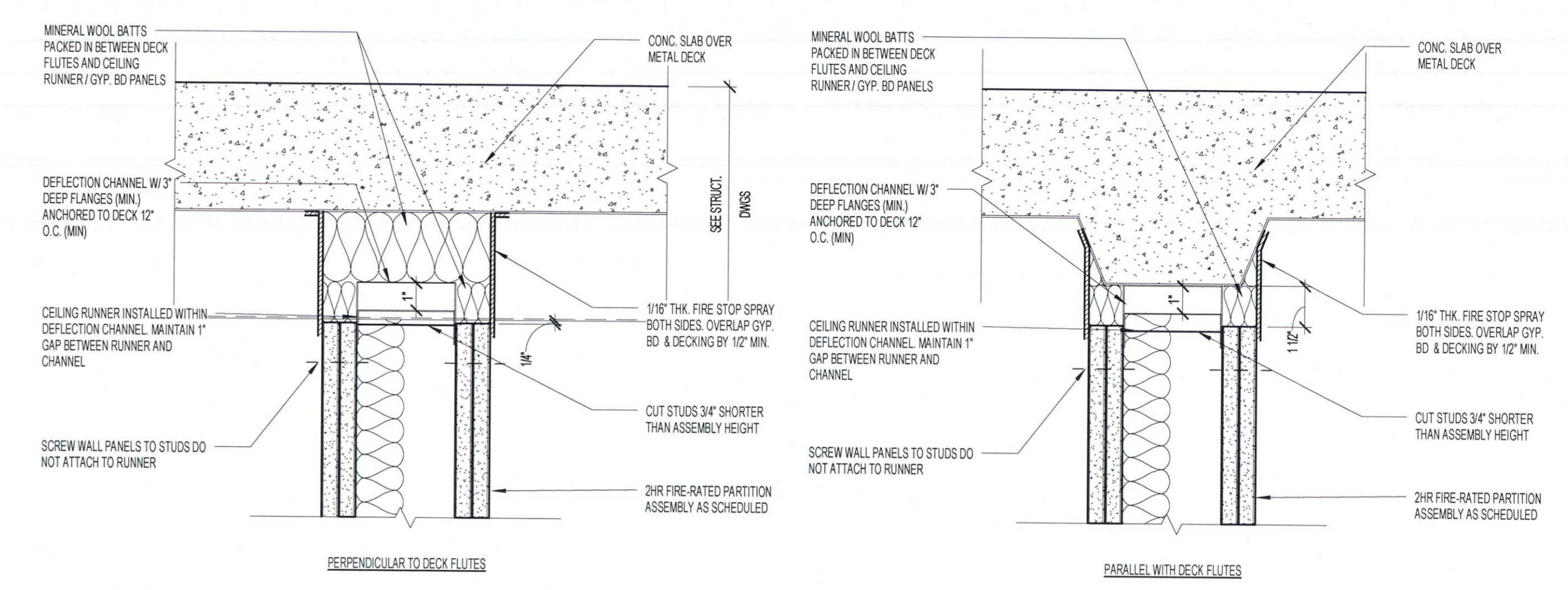
4 PARTITION HEAD DETAIL 3" = 1'-0" 2 HR FIRE-RATED ASSEMBLY UL DESIGN HW-D-0107
