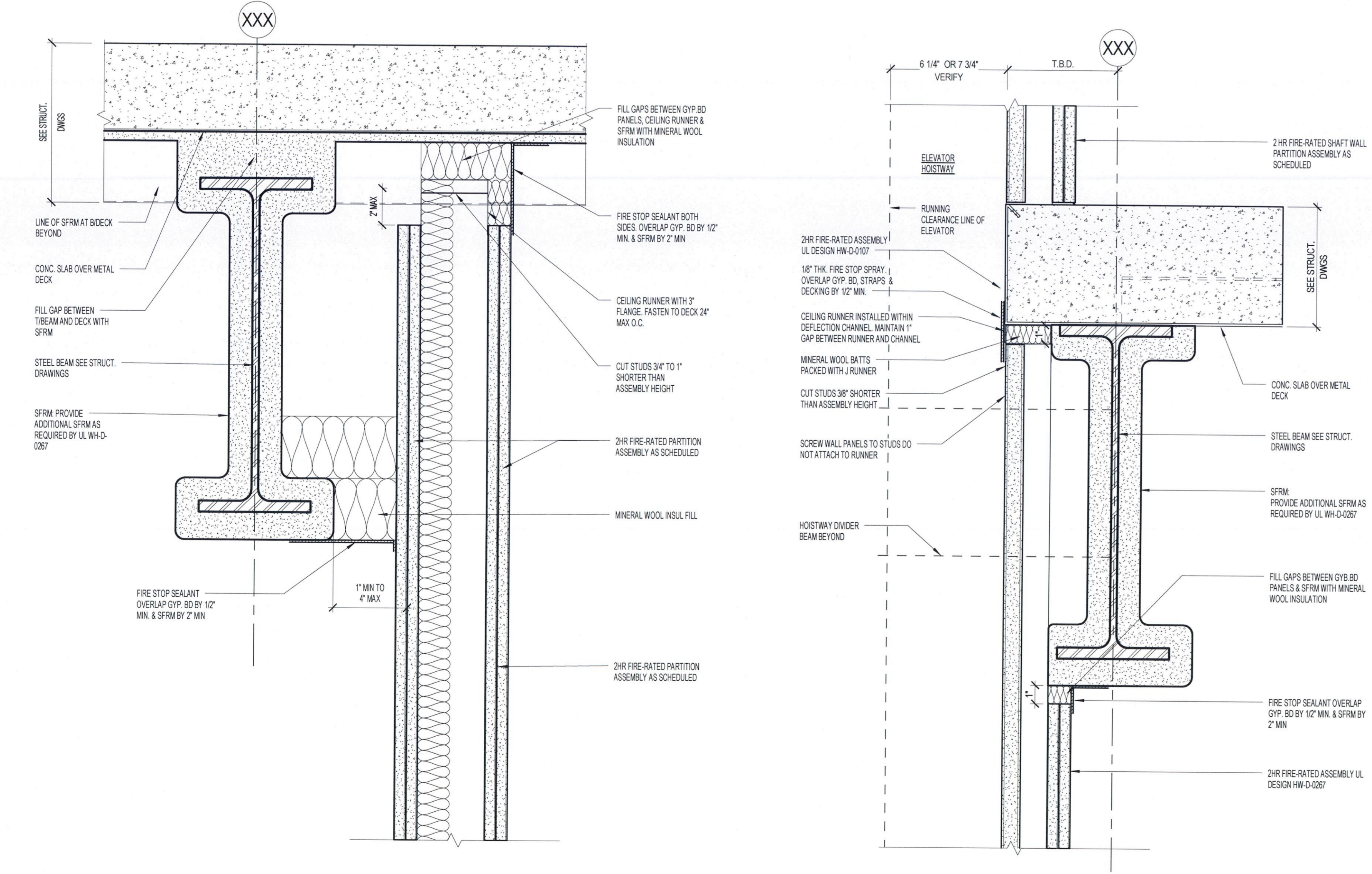
7 PARTITION HEAD DETAIL 3" = 1'-0" 2 HR FIRE-RATED ASSEMBLY UL DESIGN HW-D-0384
