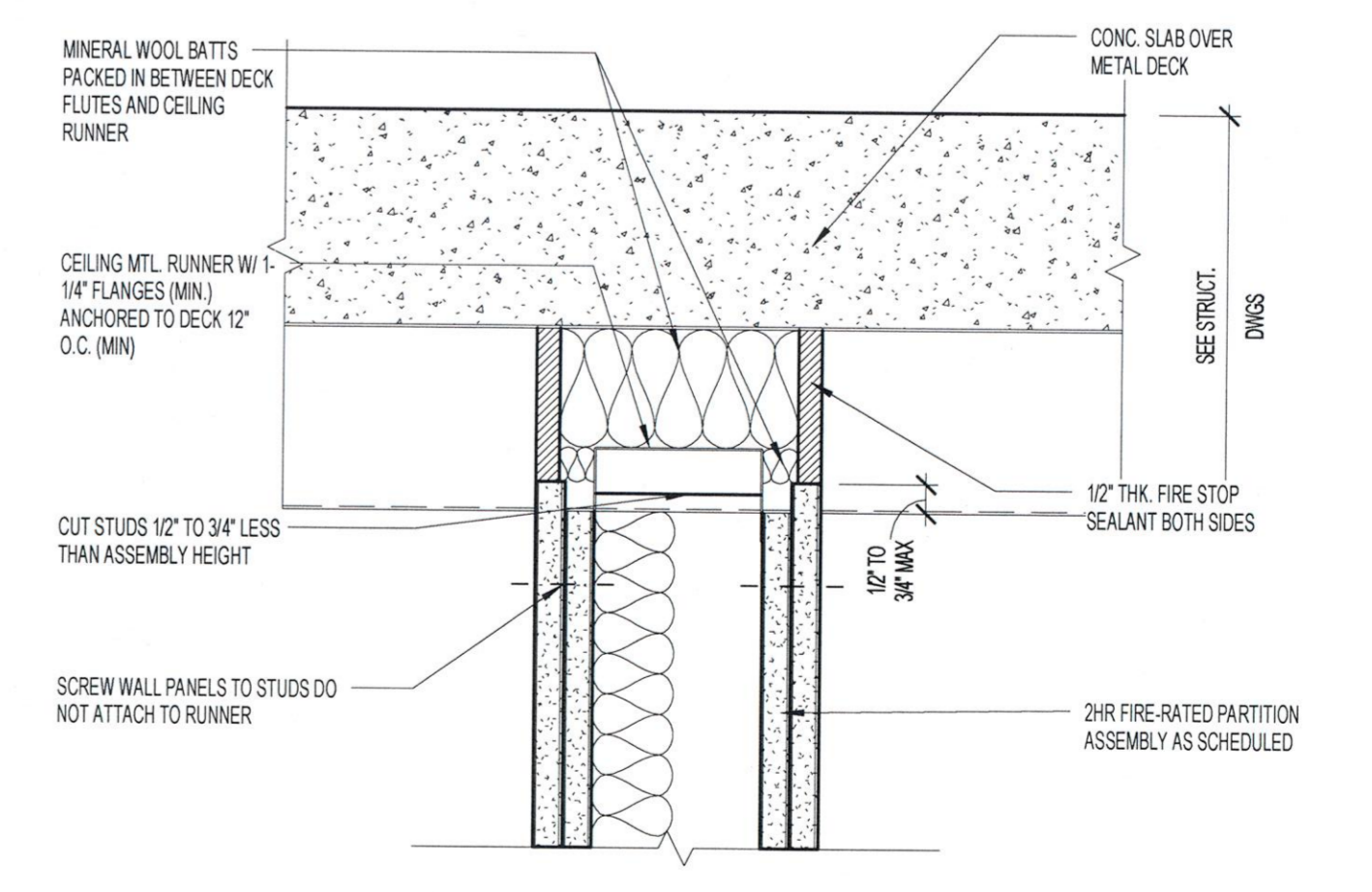
1 PARTITION HEAD DETAIL 3" = 1'-0" 2 HR FIRE-RATED ASSEMBLY UL DESIGN HW-D-0046
