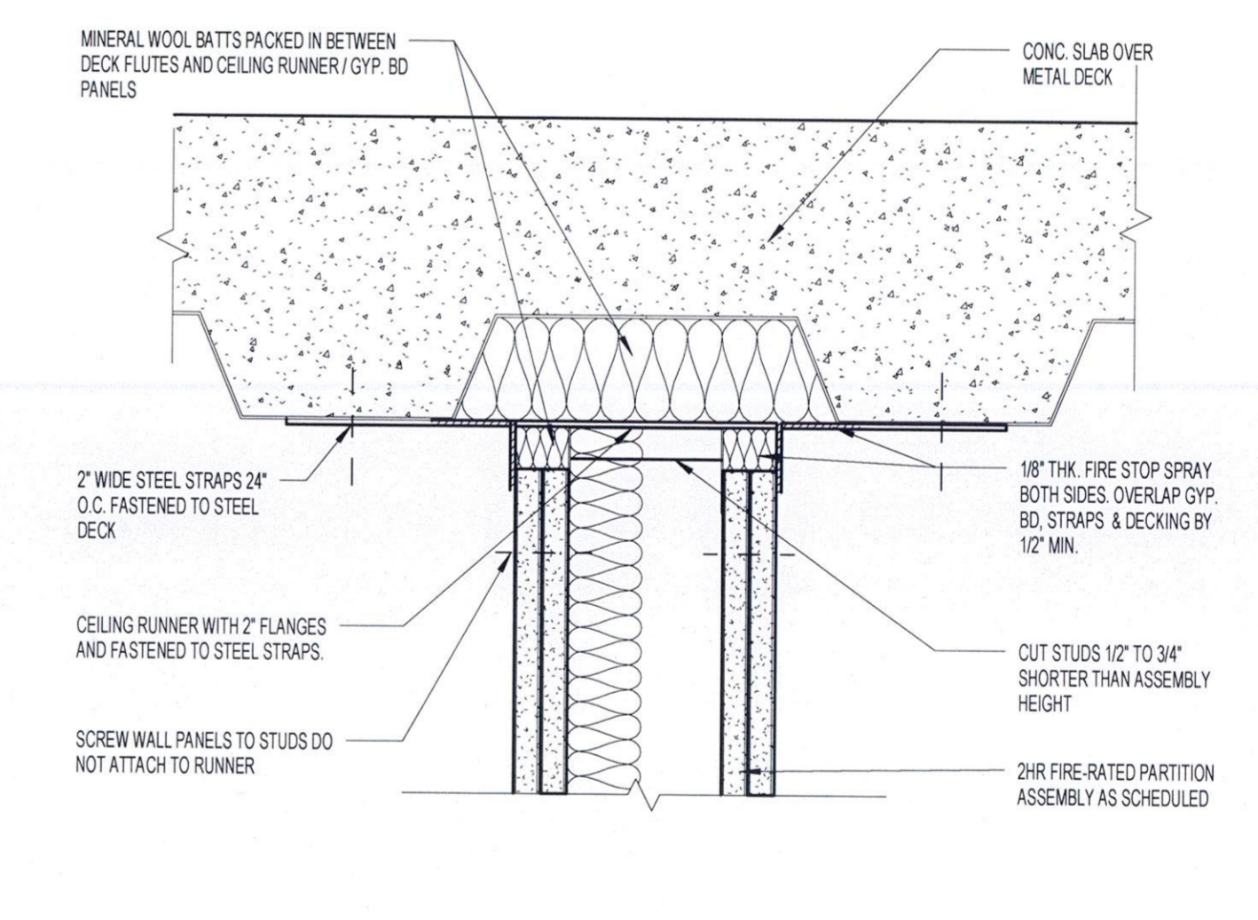
2 PARTITION HEAD DETAIL 3" = 1'-0" 2 HR FIRE-RATED ASSEMBLY UL DESIGN HW-D-0264
