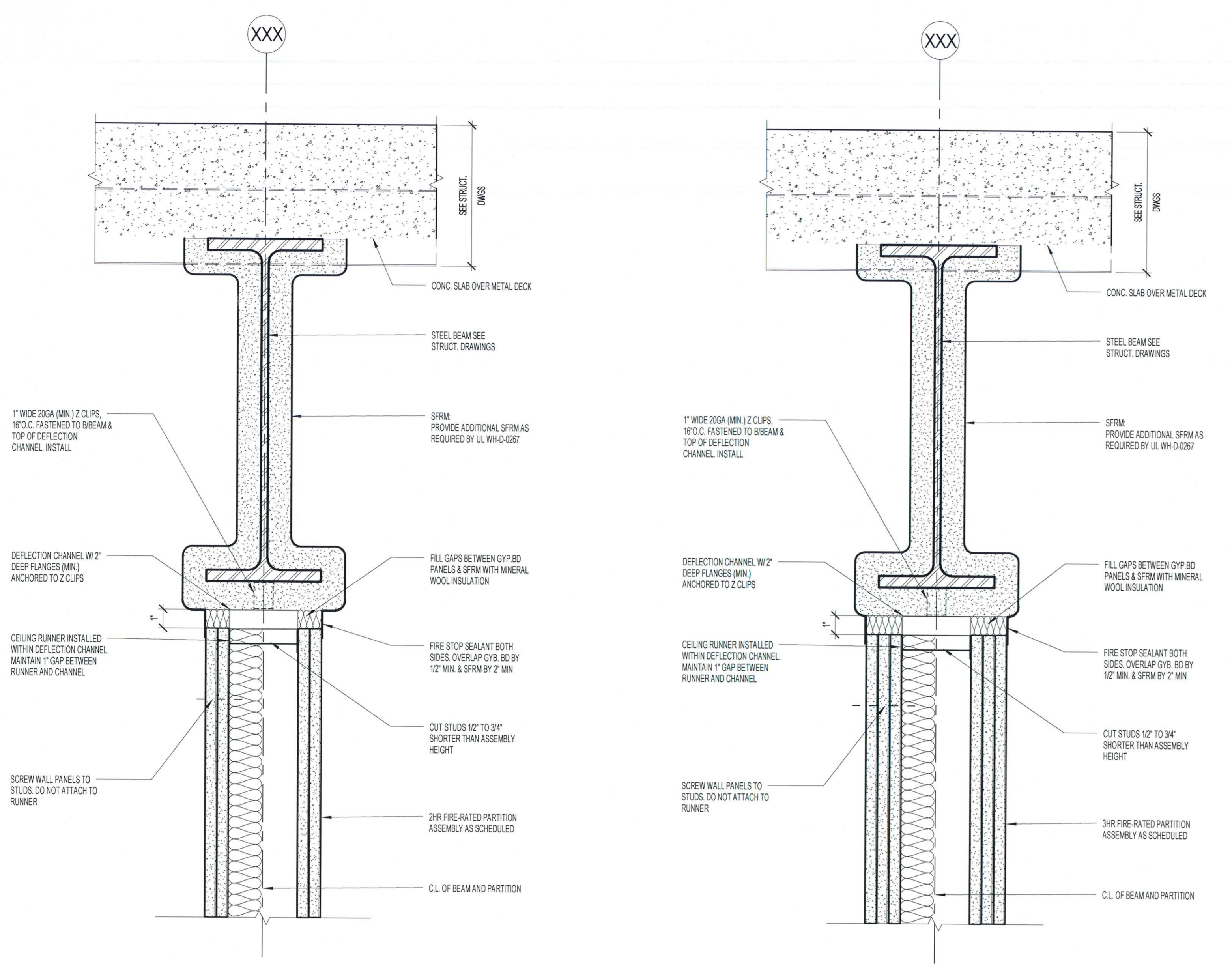
6 PARTITION HEAD DETAIL 3" = 1'-0" 2 HR FIRE-RATED ASSEMBLY UL DESIGN HW-D-0267
