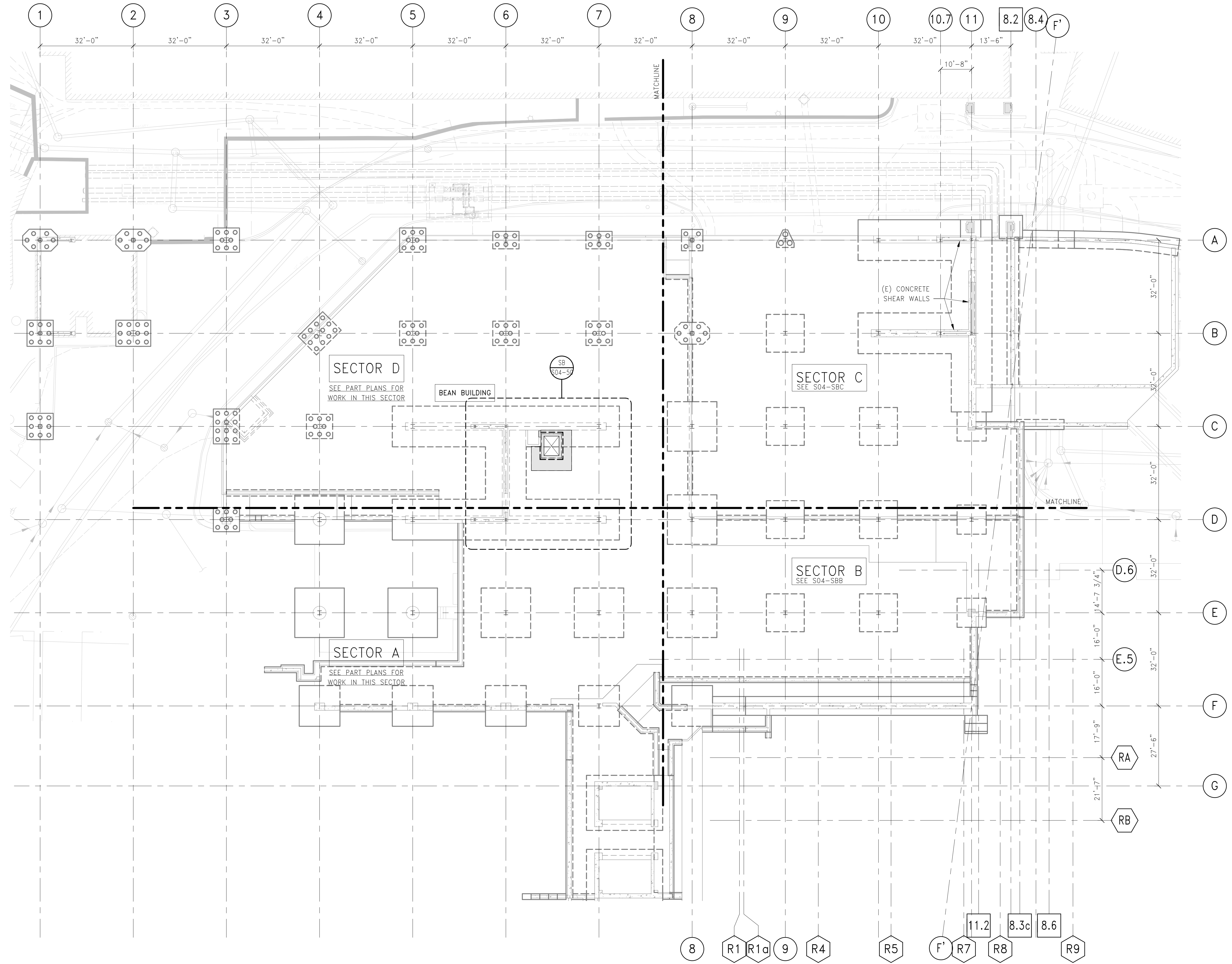
SUB-BASEMENT / FOUNDATION PLAN 1/16" = 1'-0"
