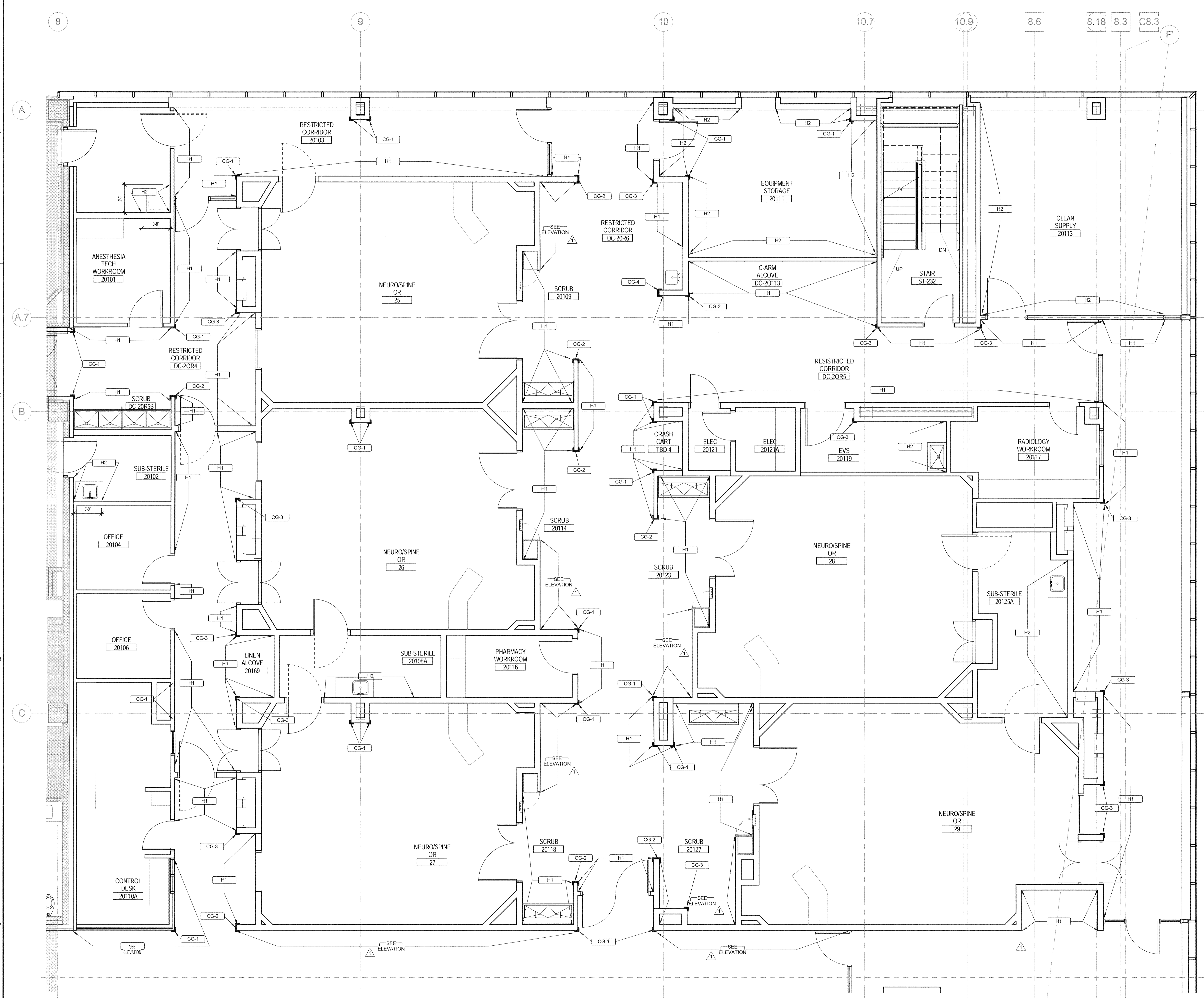
LEVEL 2 - WALL PROTECTION PLAN - SECTOR C A1 1/4" = 1'-0"
