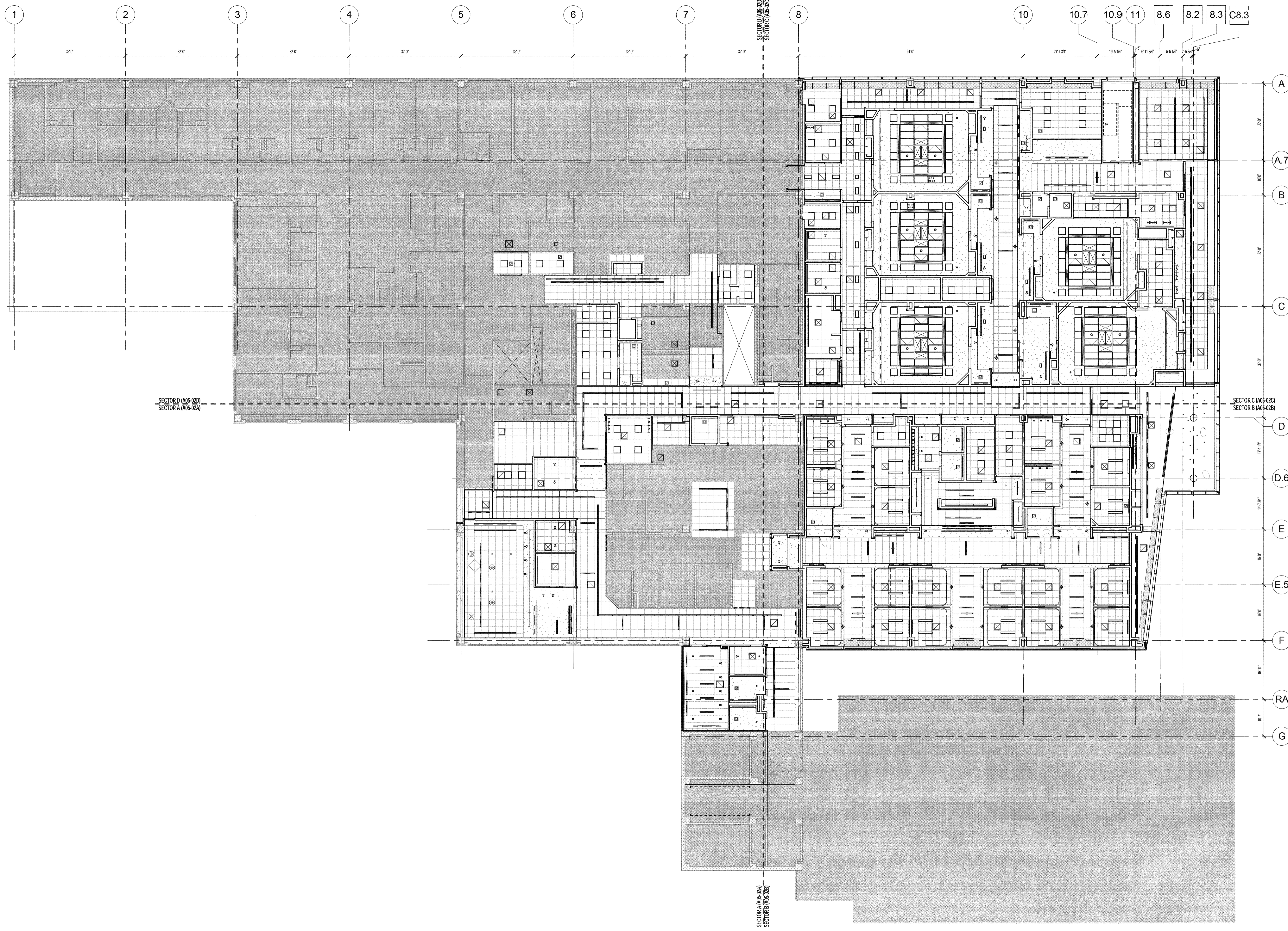
A1 BEAN LEVEL 2 OVERAL RCP 3/32" = 1'-0"
