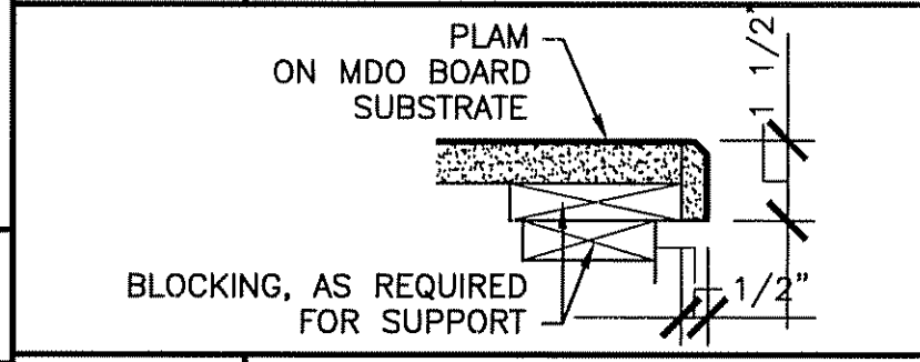
C5 CASEWORK DETAIL
