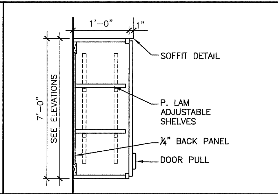
D3 CASEWORK DETAIL
