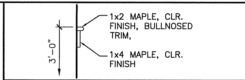
D5 CASEWORK DETAIL
