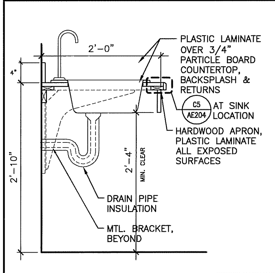
A1 CASEWORK DETAIL
