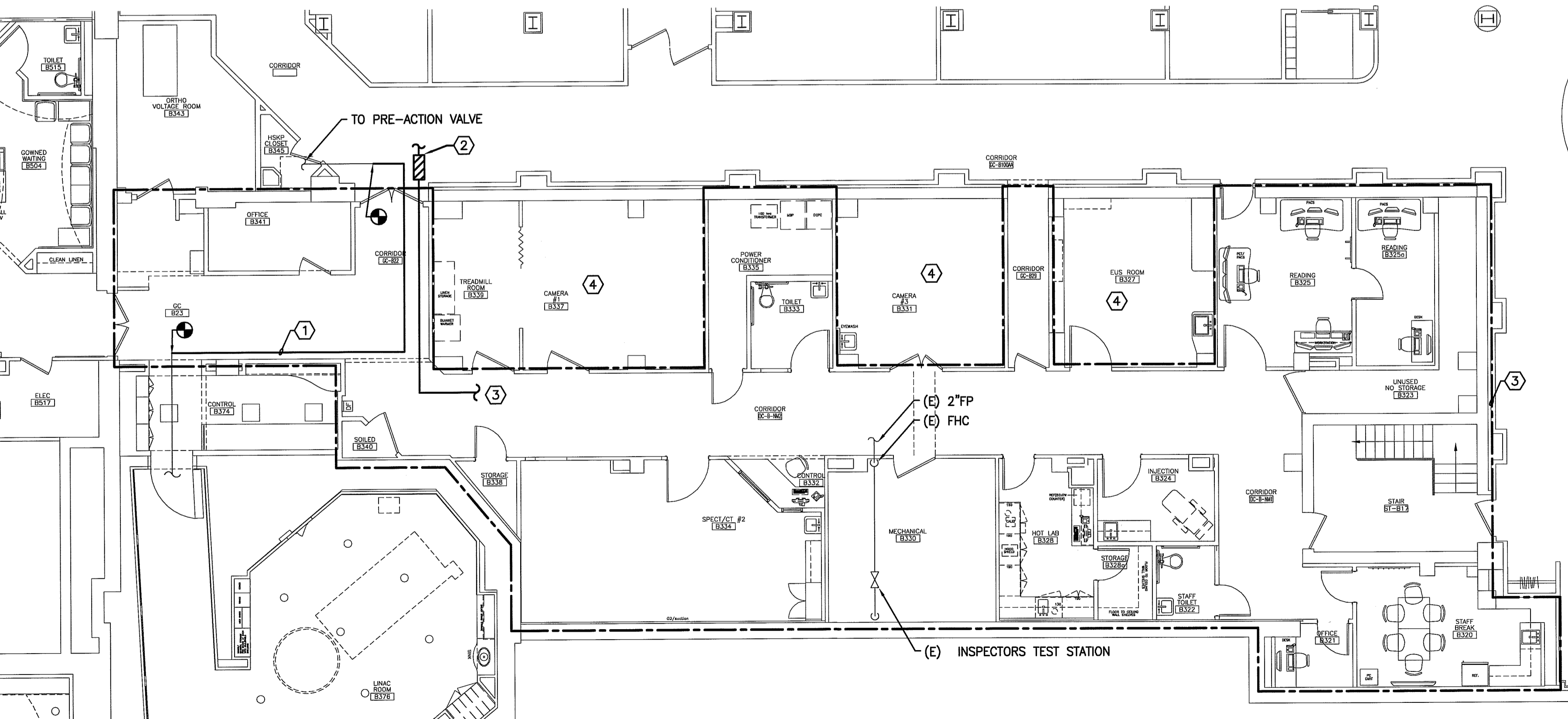
A1 FIRE PROTECTION NEW WORK PLAN
