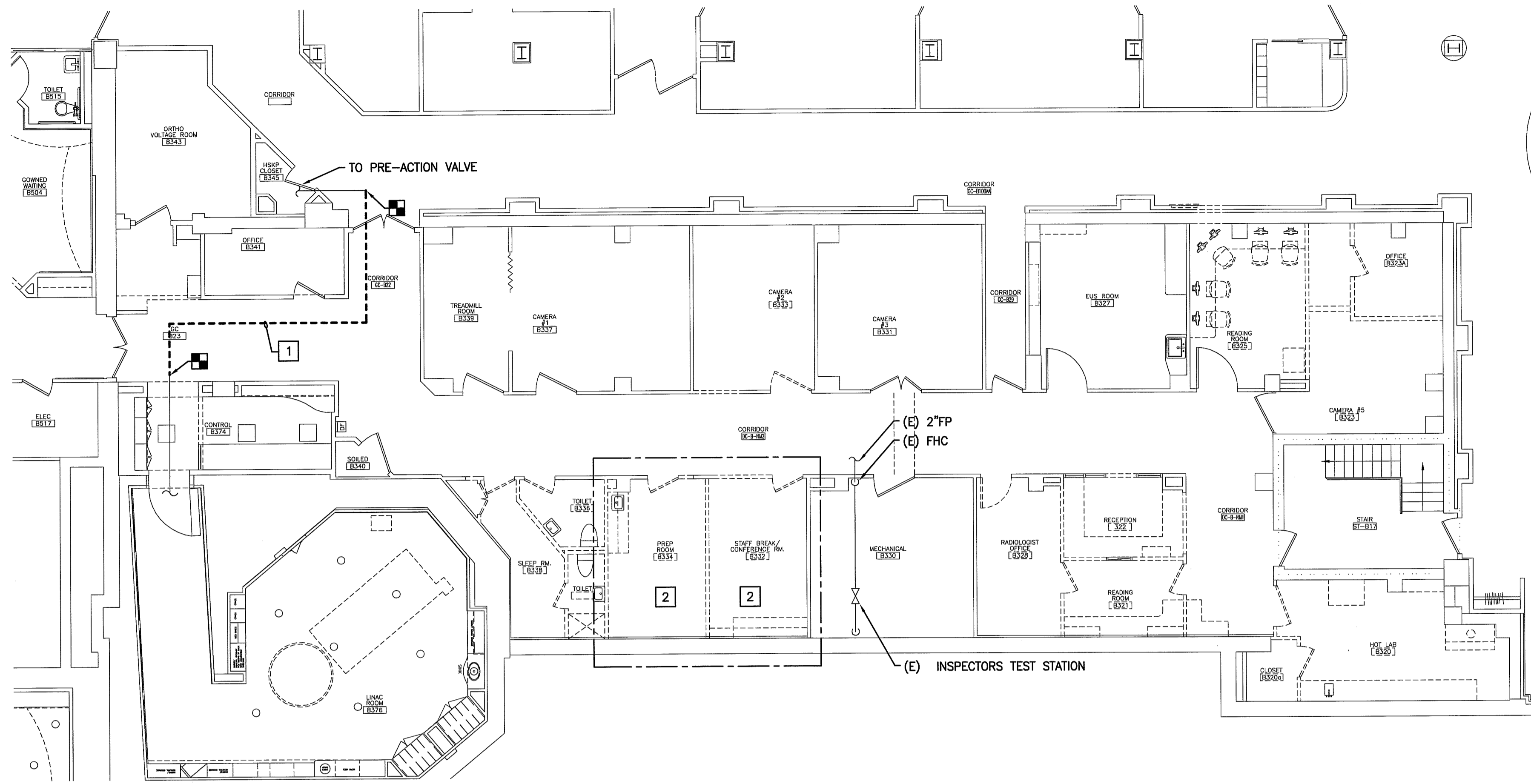
G1 FIRE PROTECTION DEMOLITION PLAN
