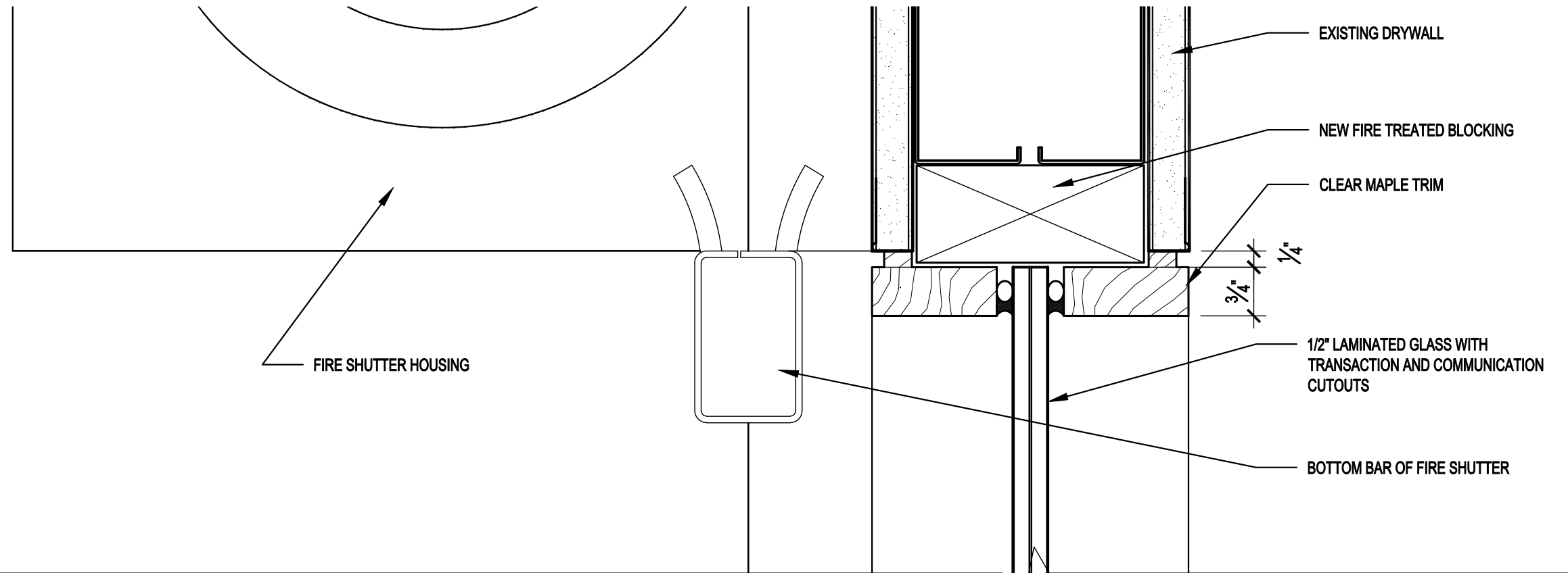
1 RECEPTION COUNTER WINDOW 1/4"=1'-0"
