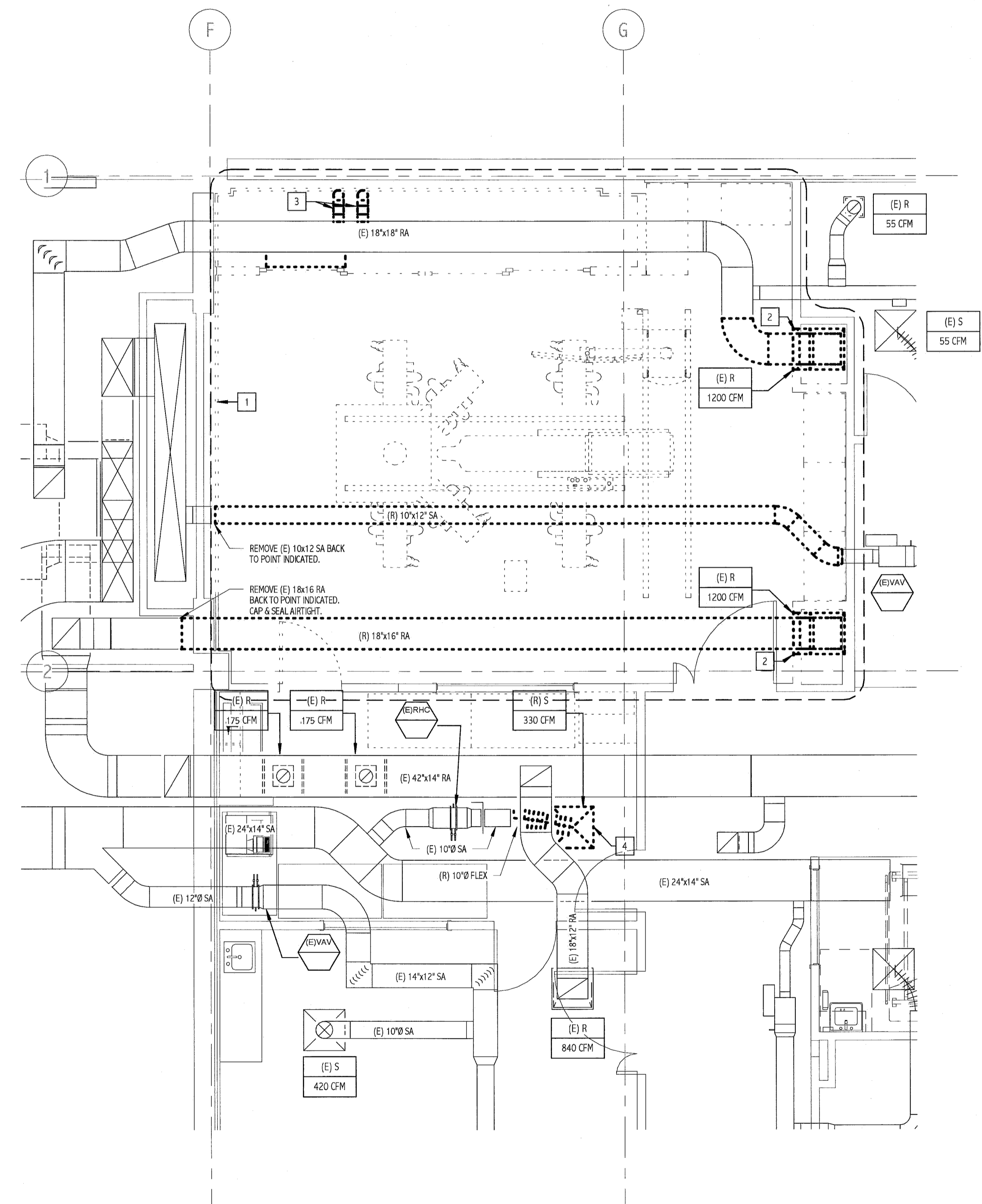
1 BASMENT DUCTWORK DEMOLITION PLAN 1/4" = 1'-0"
