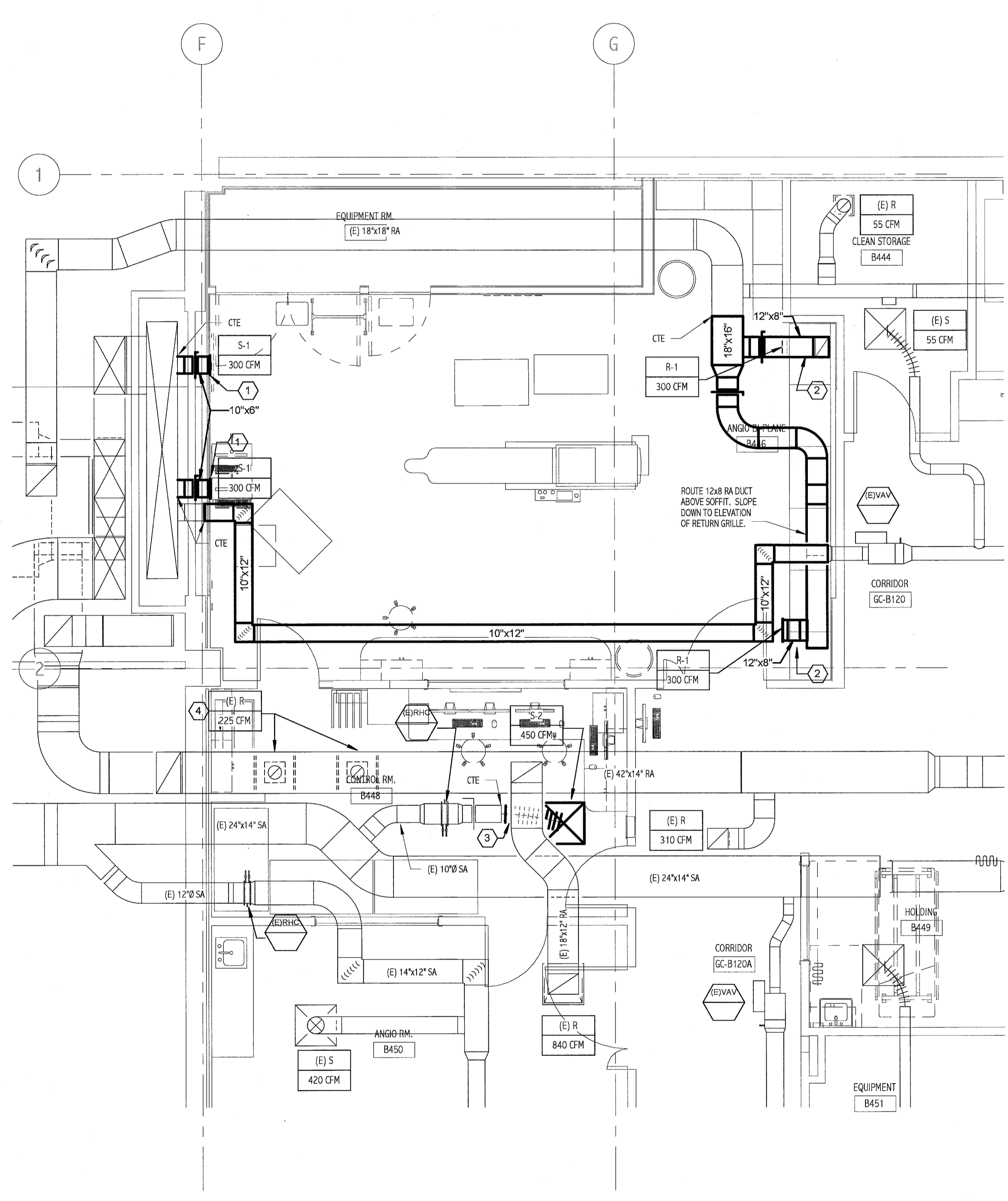
2 BASEMENT DUCTWORK PLAN 1/4" = 1'-0"
