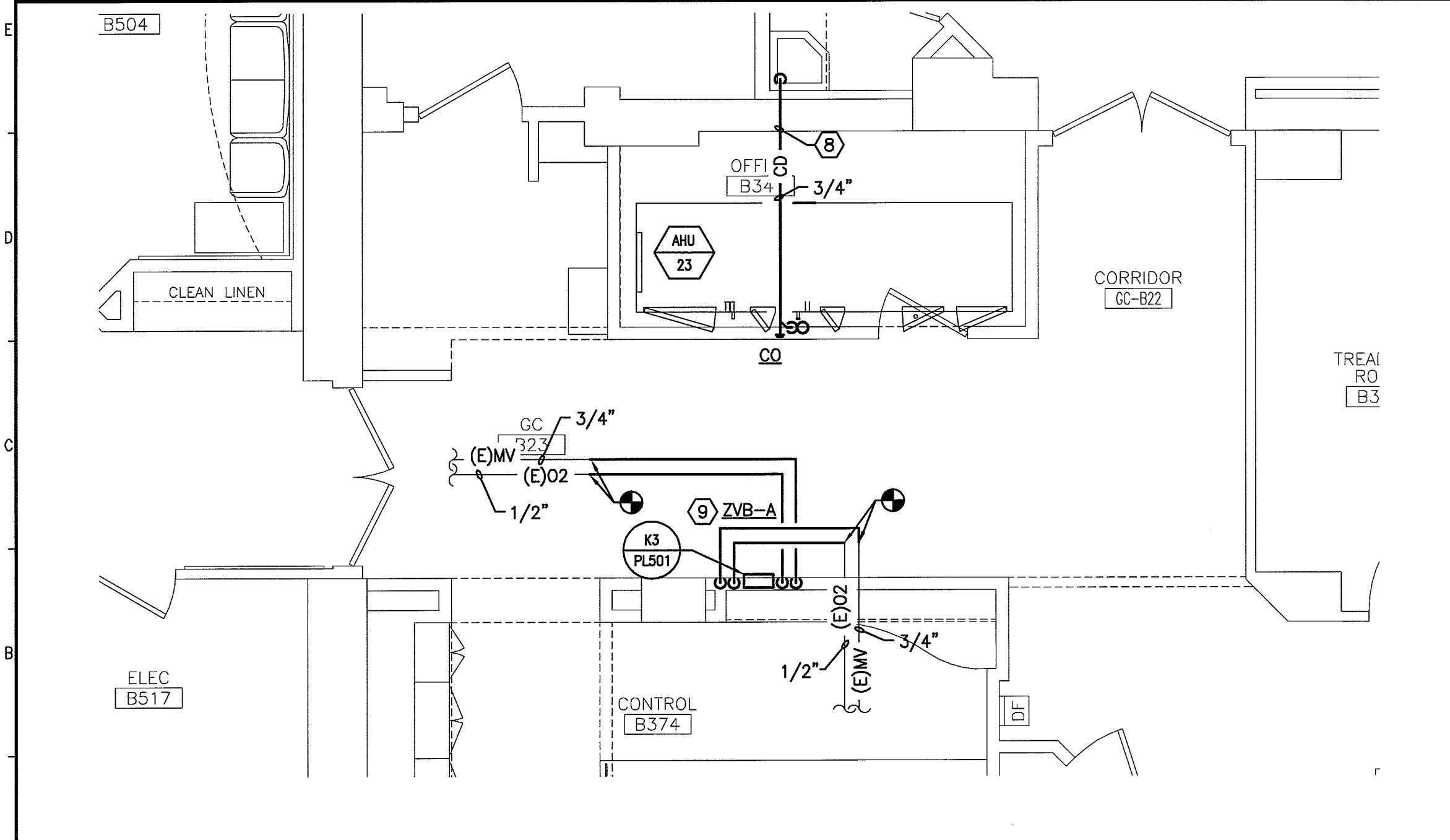
A1 PLUMBING PART PLAN
