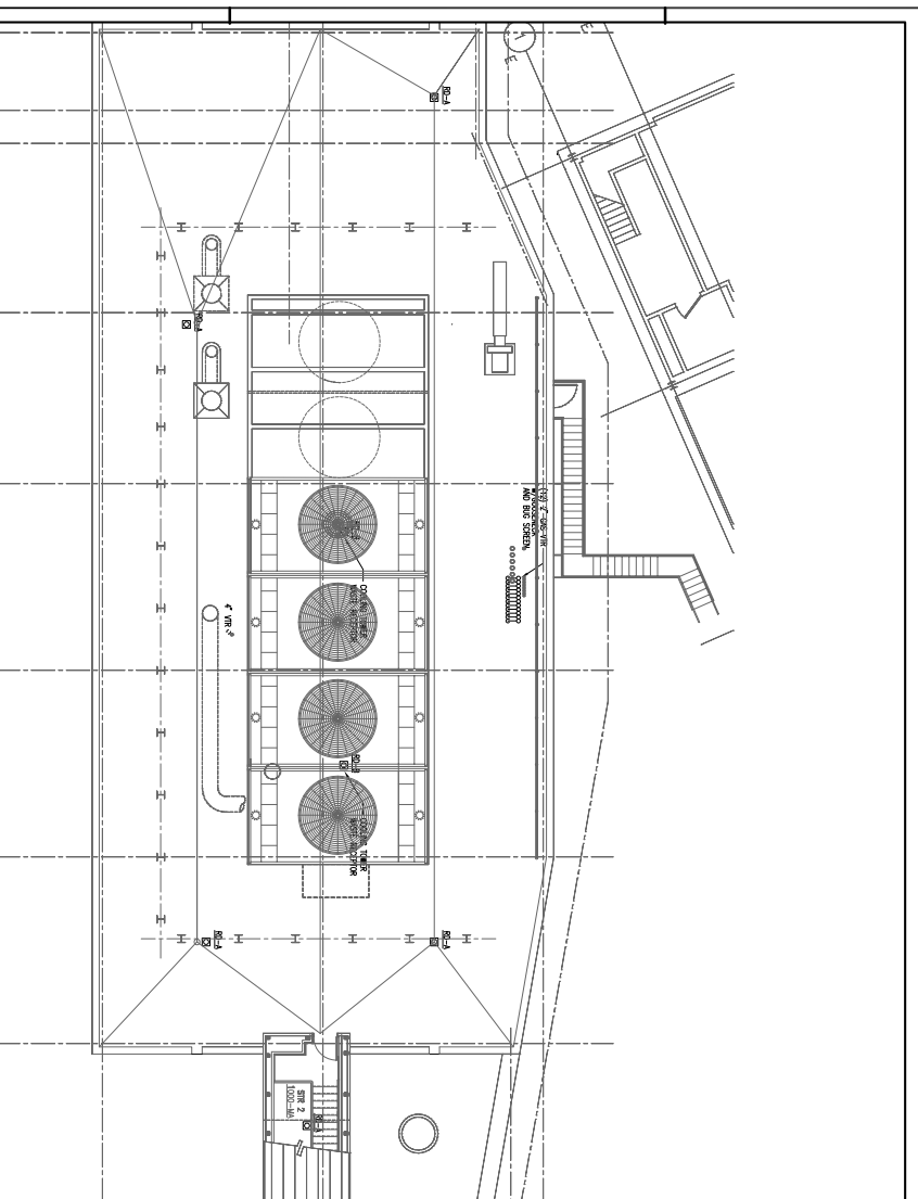
ROOF PLAN
