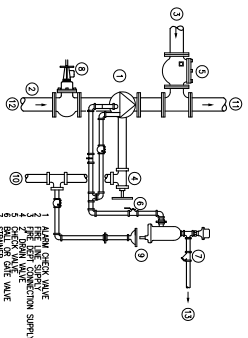
3 ALARM CHECK VALVE DETAIL SCALE: NS
