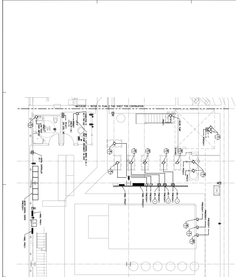
1 LEVEL 1 POWER AND SIGNAL PLAN - BOILER PLANT 1/8"=1'-0"
