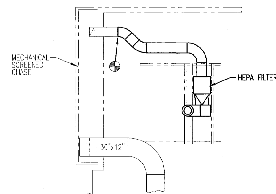
ROOF PART PLAN SCALE: 1/8"=1'-0"
