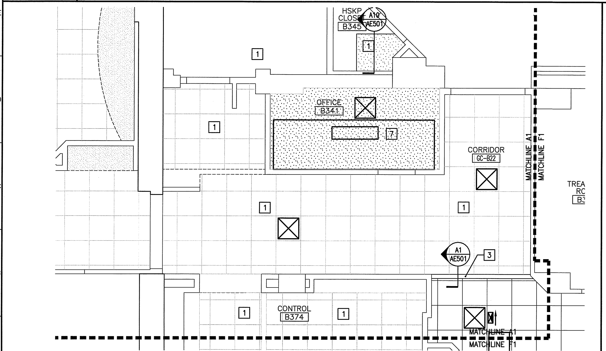
A1 REFLECTED CEILING PLAN
