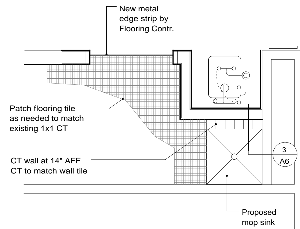
2 Partial Flooring Work @ Rm. #5130 1/2" = 1'-0"
