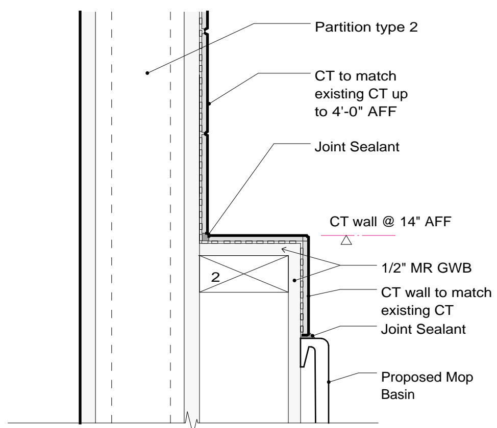
3 Tile Detail at Mop Basin 3" = 1'-0"
