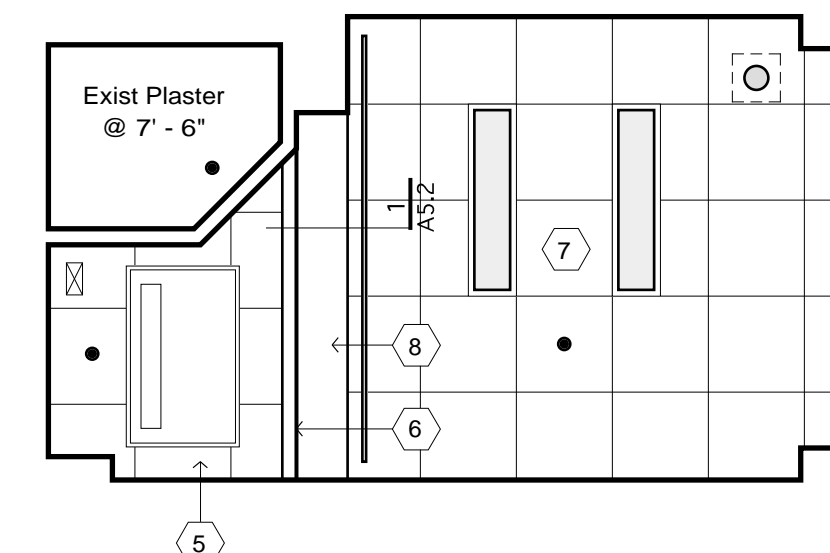
Typical Patient Room Ceiling Plan
