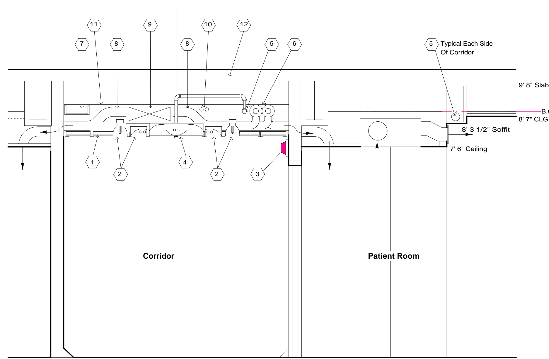
Corridor Cross Section
