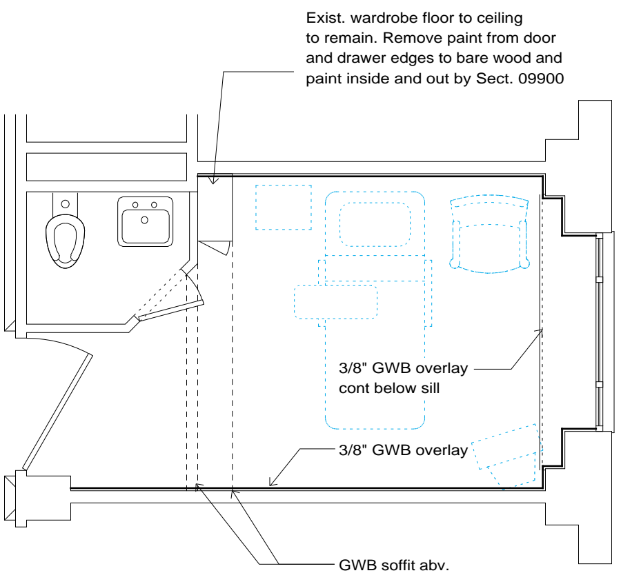
Plan at Typical Patient Room
