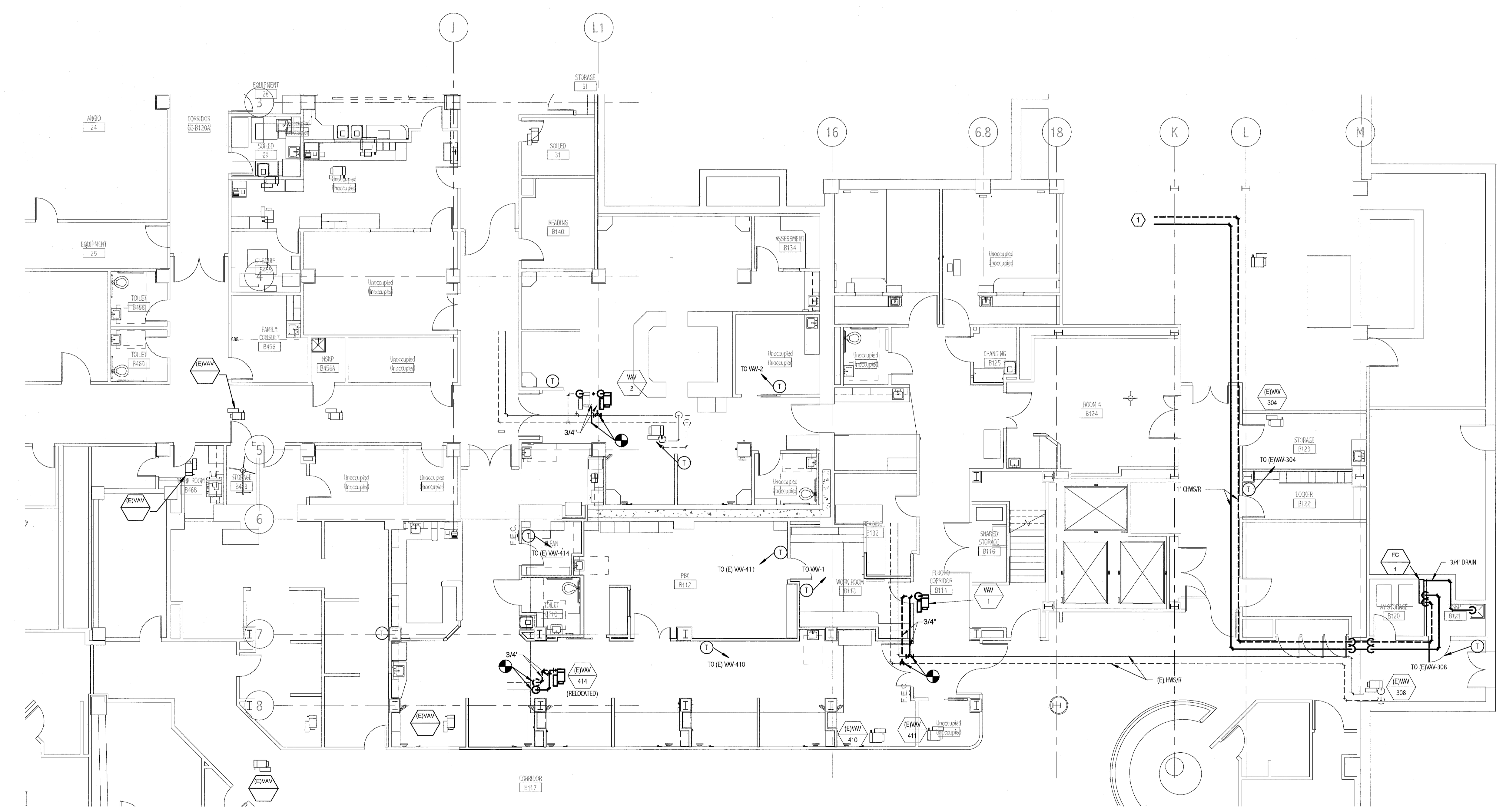
① BASEMENT LEVEL PIPING PLAN 1/8" = 1'-0"
