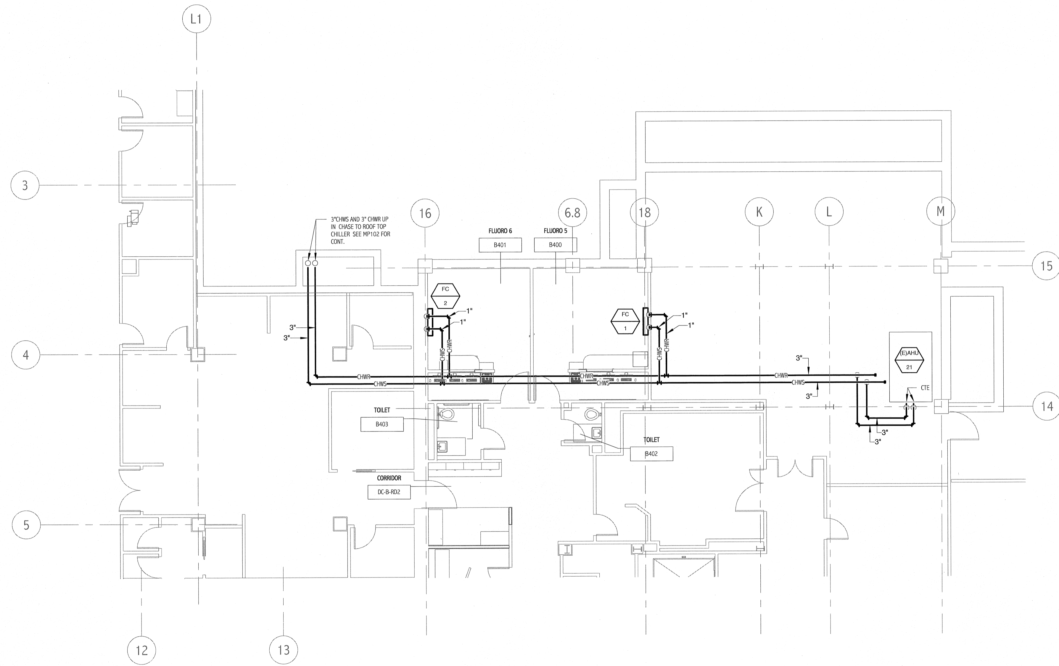
1 FLUORO HVAC PIPING PLAN 1/8" = 1'-0"
