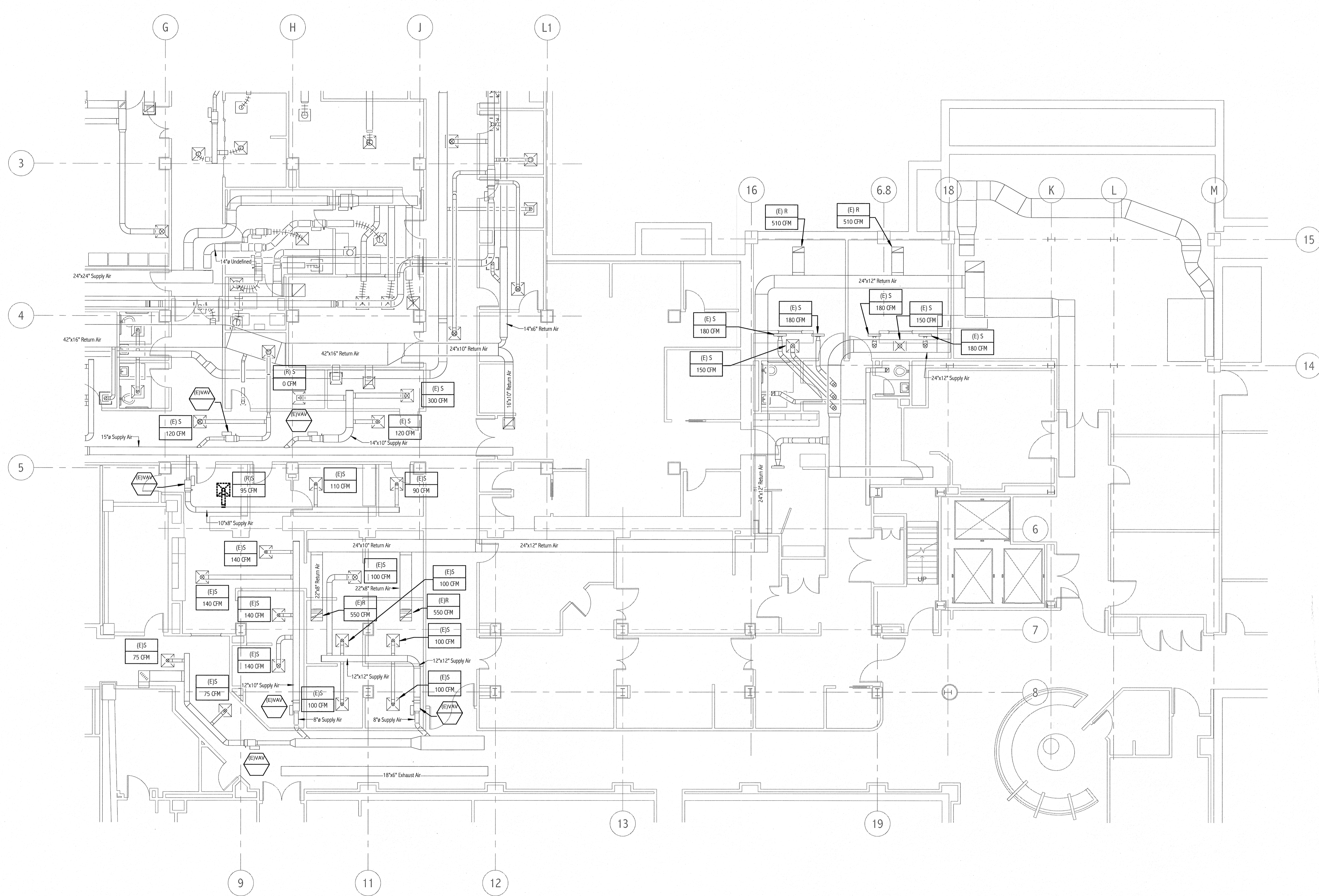
① FLUORO DEMOLITION PLAN 1/8" = 1'-0"
