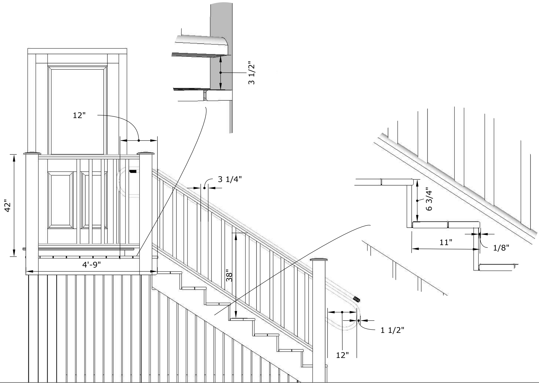
North Elevation w Details (Scale 1/2":1')
