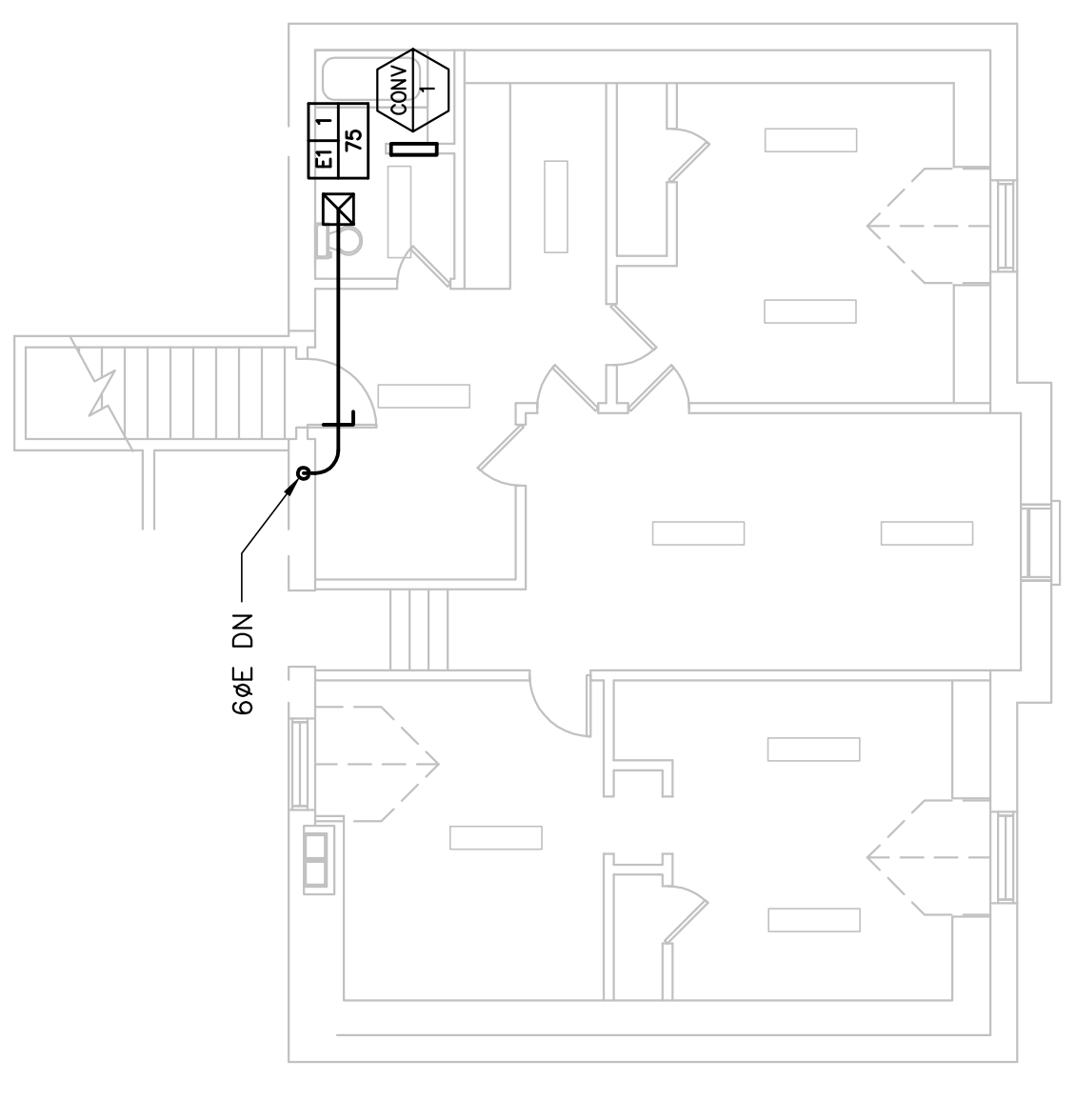
MECHANICAL PLAN ~ THIRD FLOOR
