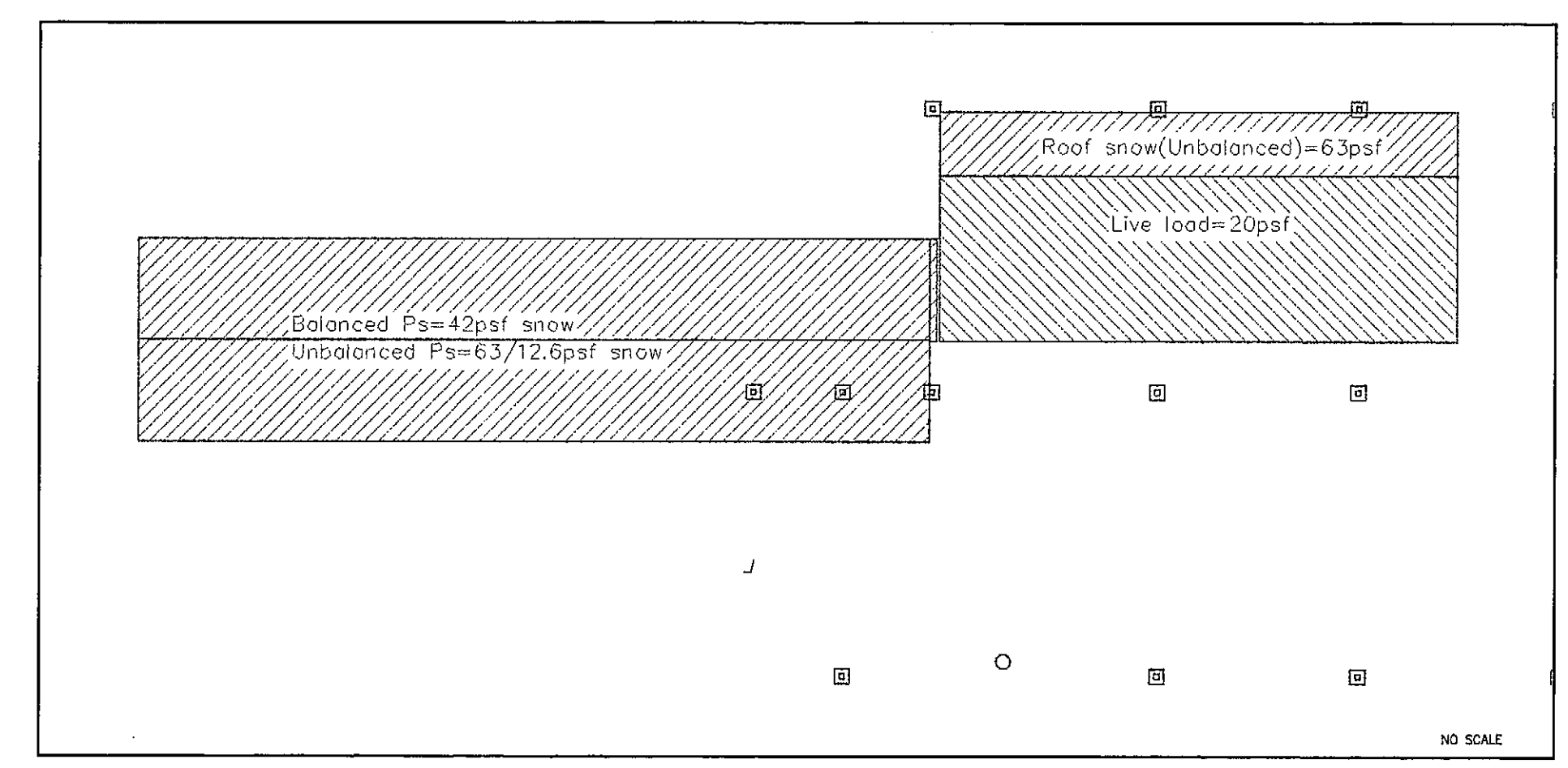
LOAD PLAN
