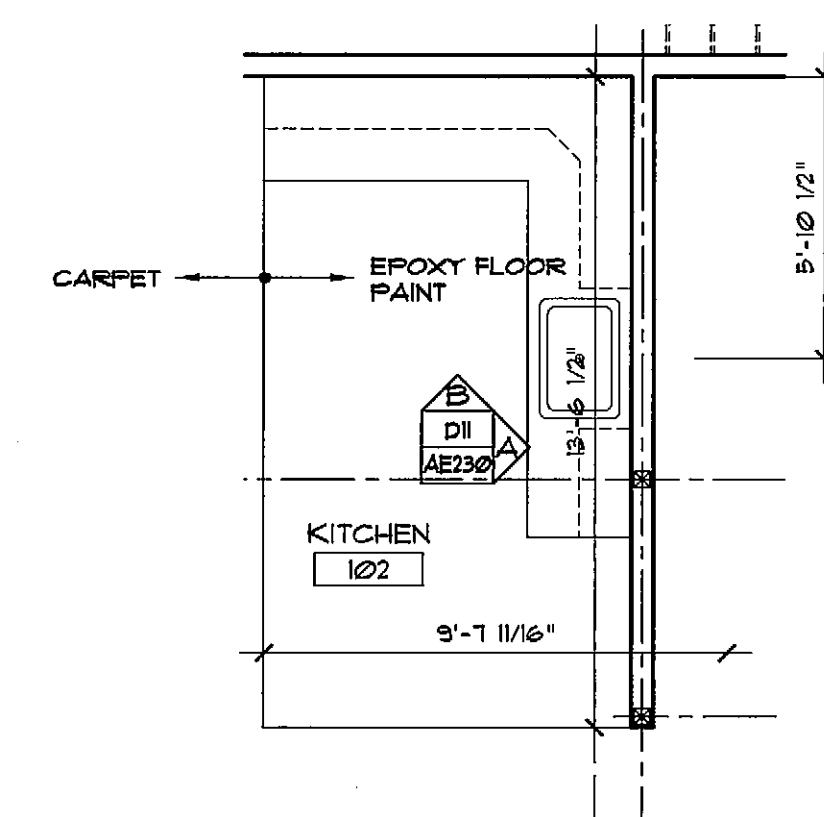
A1 ENLARGED KITCHEN PLAN SCALE 1/4" = 1'-0"
