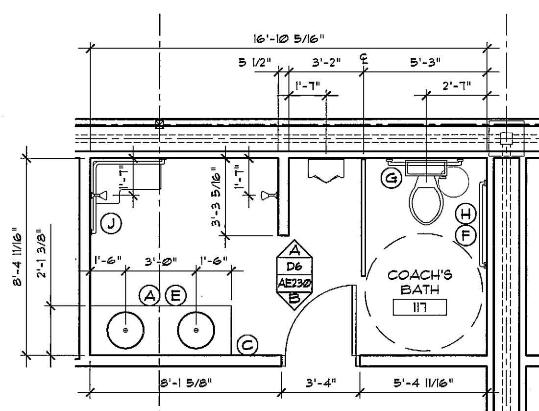
E1 ENLARGED COACH'S BATH SCALE 1/4" = 1'-0"
