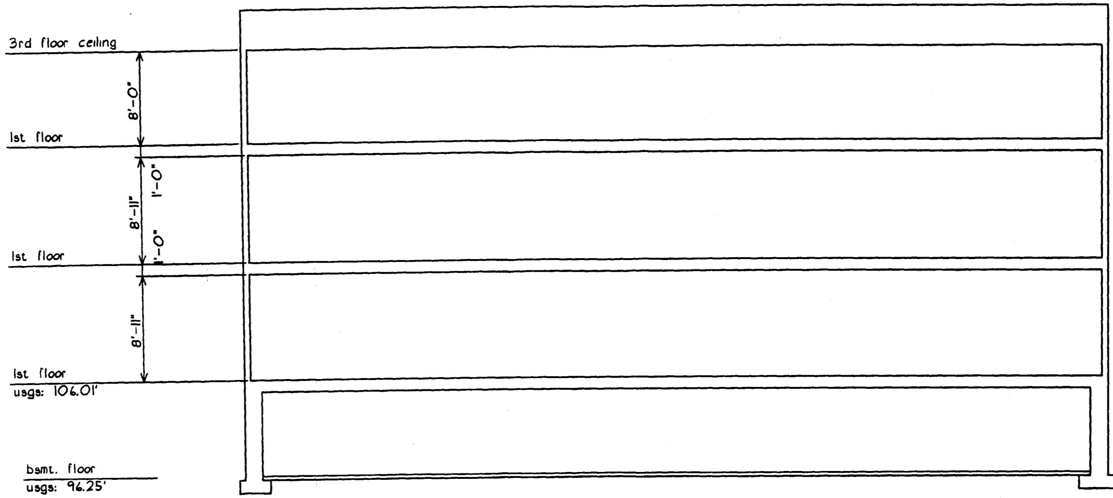
section: 1-1
