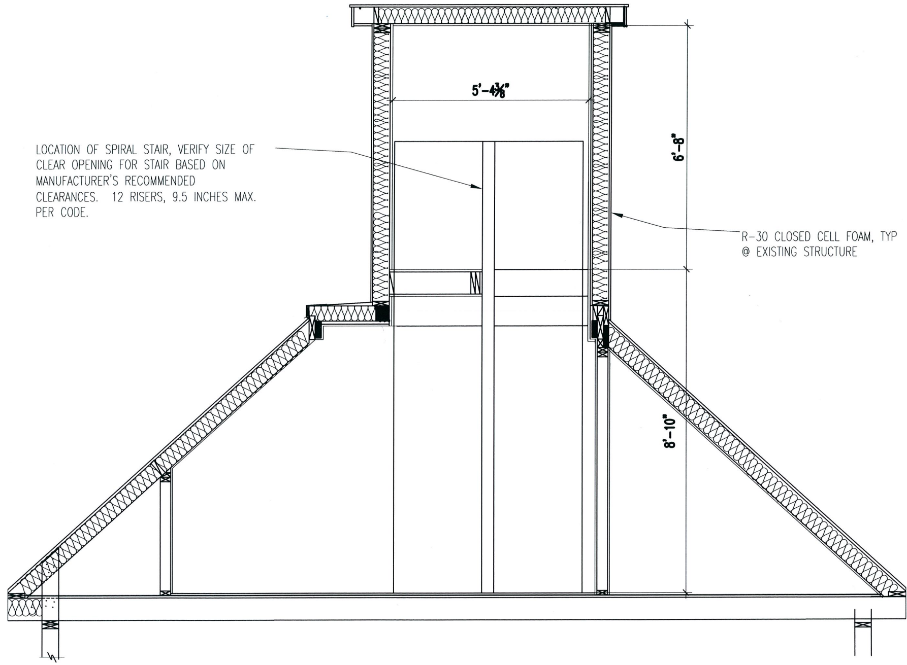
SECTION AT THE ROOFTOP HUT, LOOKING SOUTH
