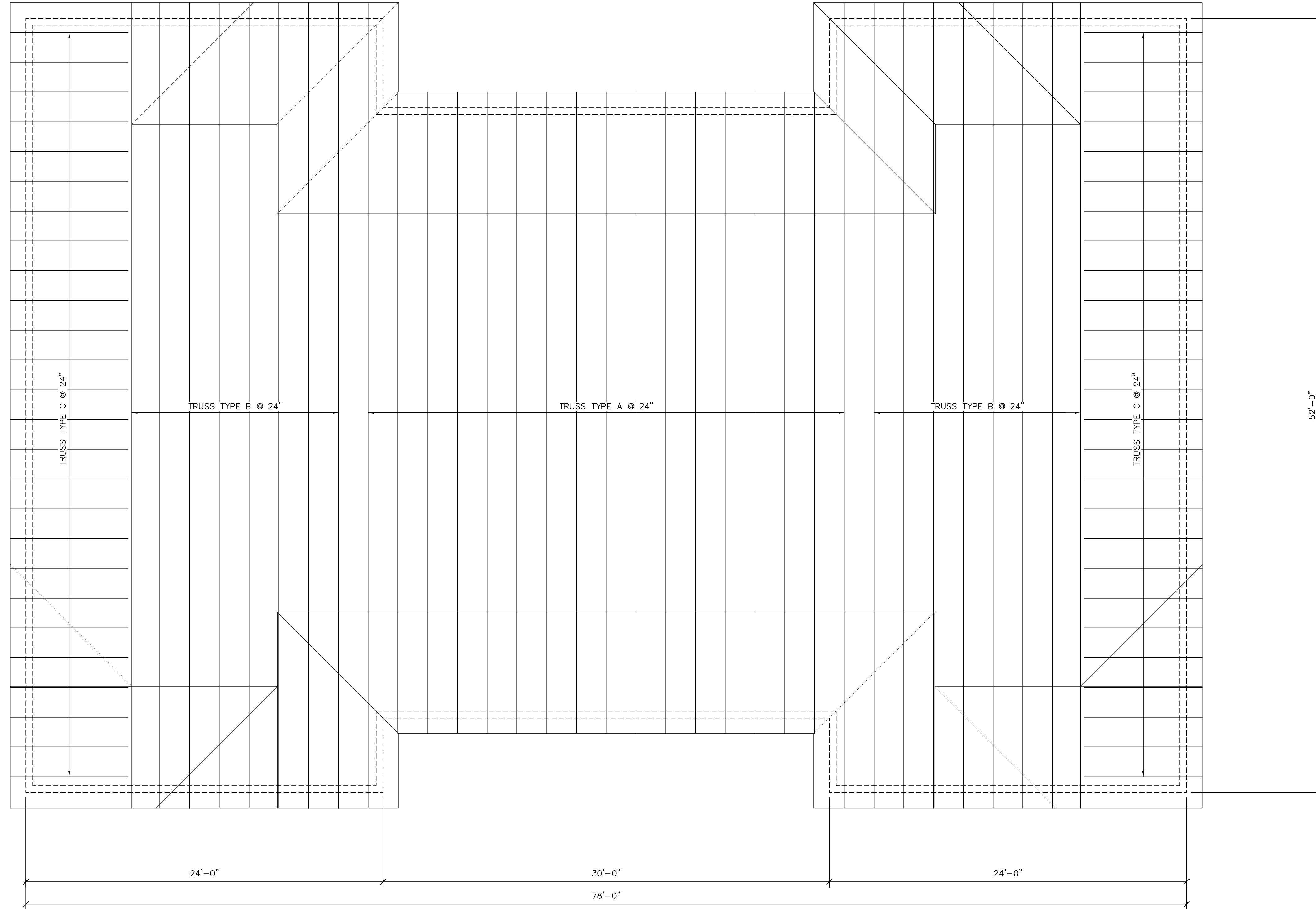
ROOF FRAMING PLAN 1/4"=1'-0"
