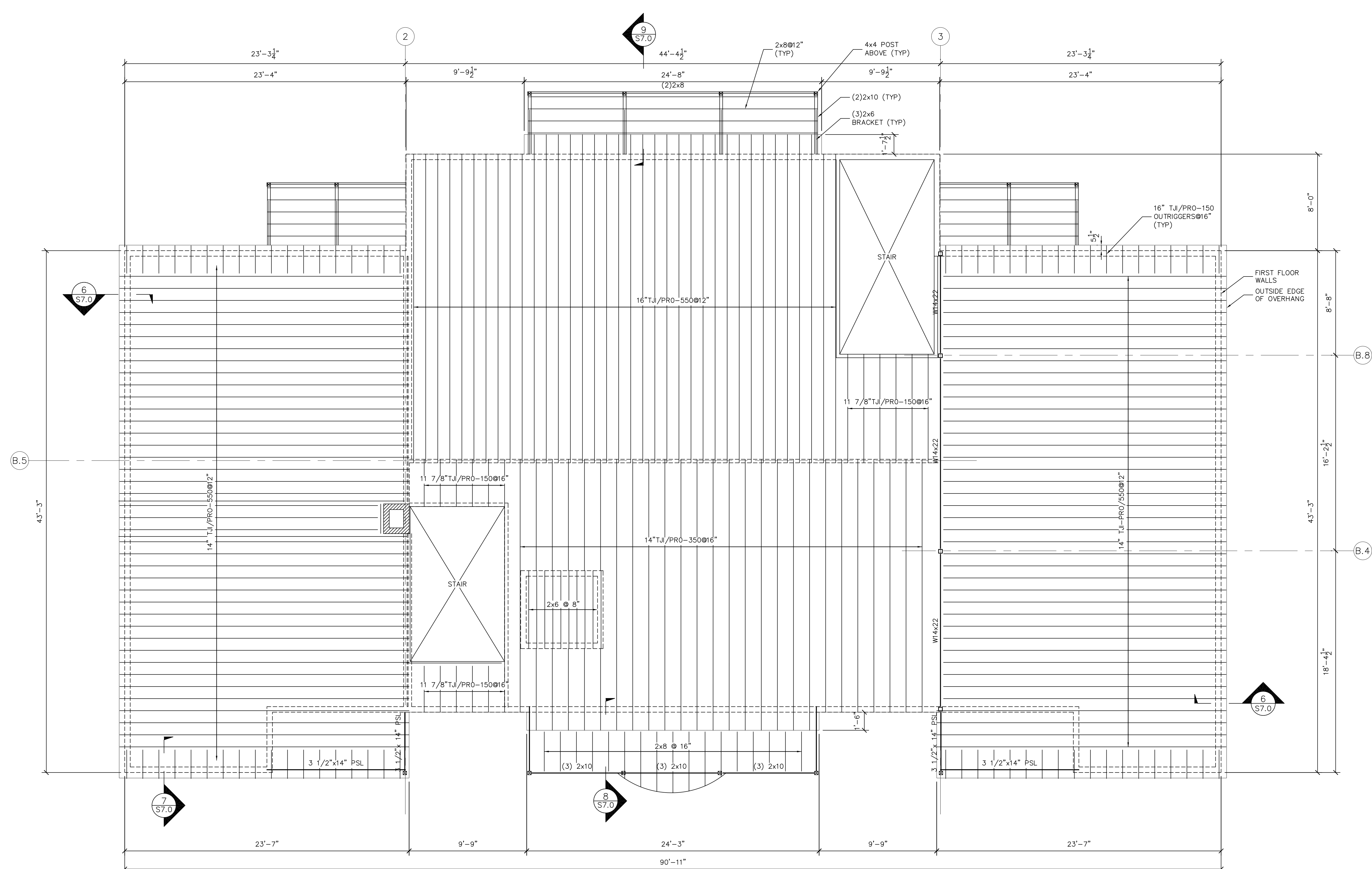
SECOND FLOOR FRAMING PLAN 1/4"=1'-0"
