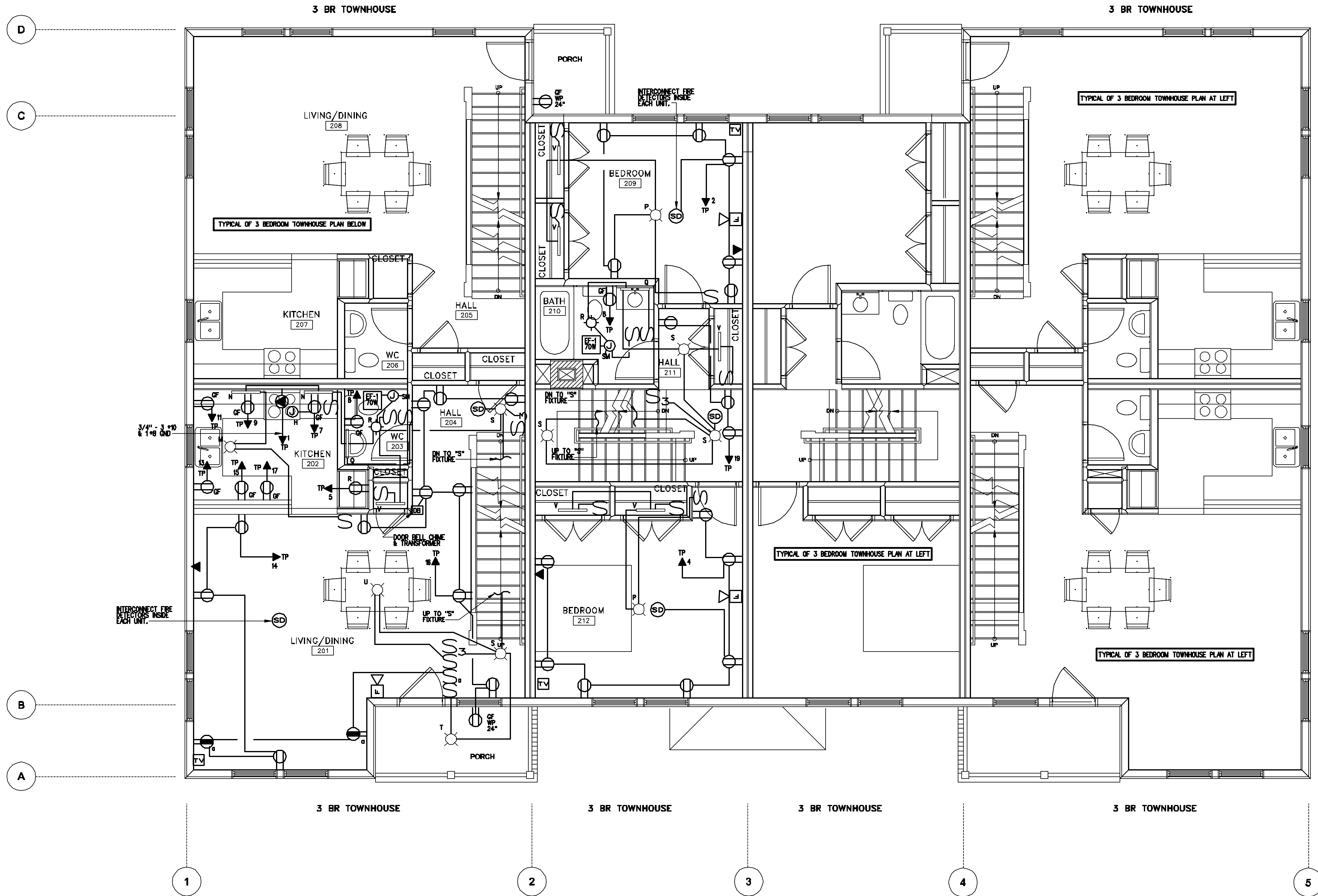
1 SECOND FLOOR ELECTRICAL PLAN BUILDING B 1/4" = 1'-0"
