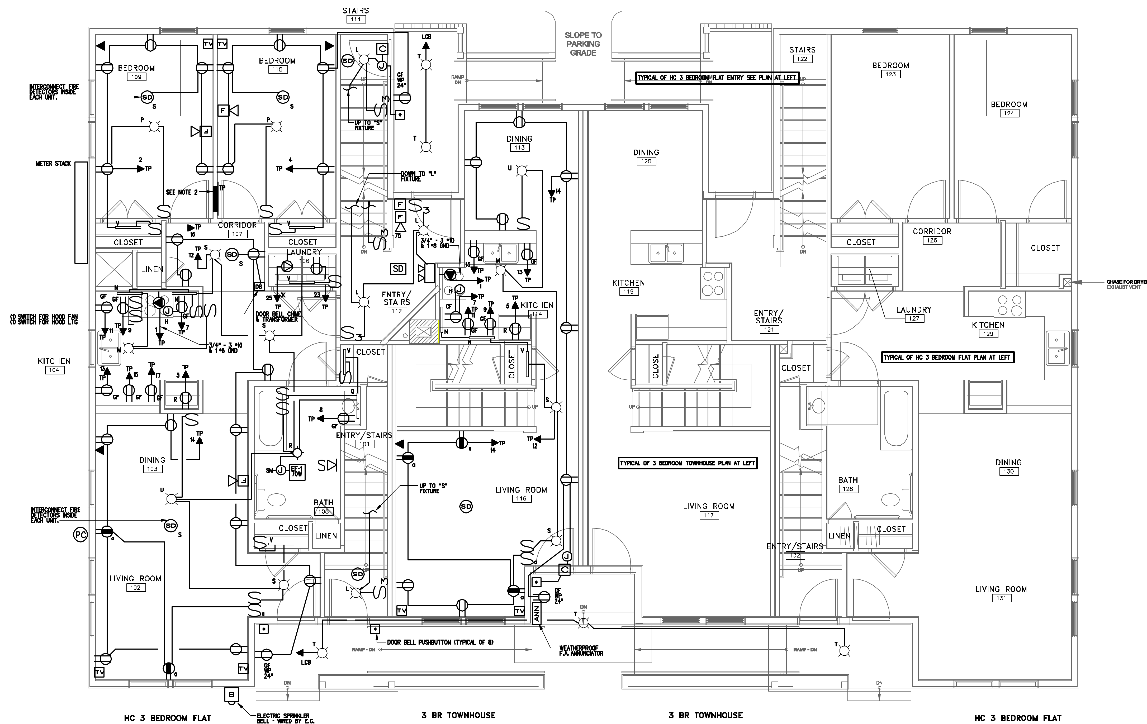
1 FIRST FLOOR ELECTRICAL PLAN BUILDING B 1/4" = 1'-0"
