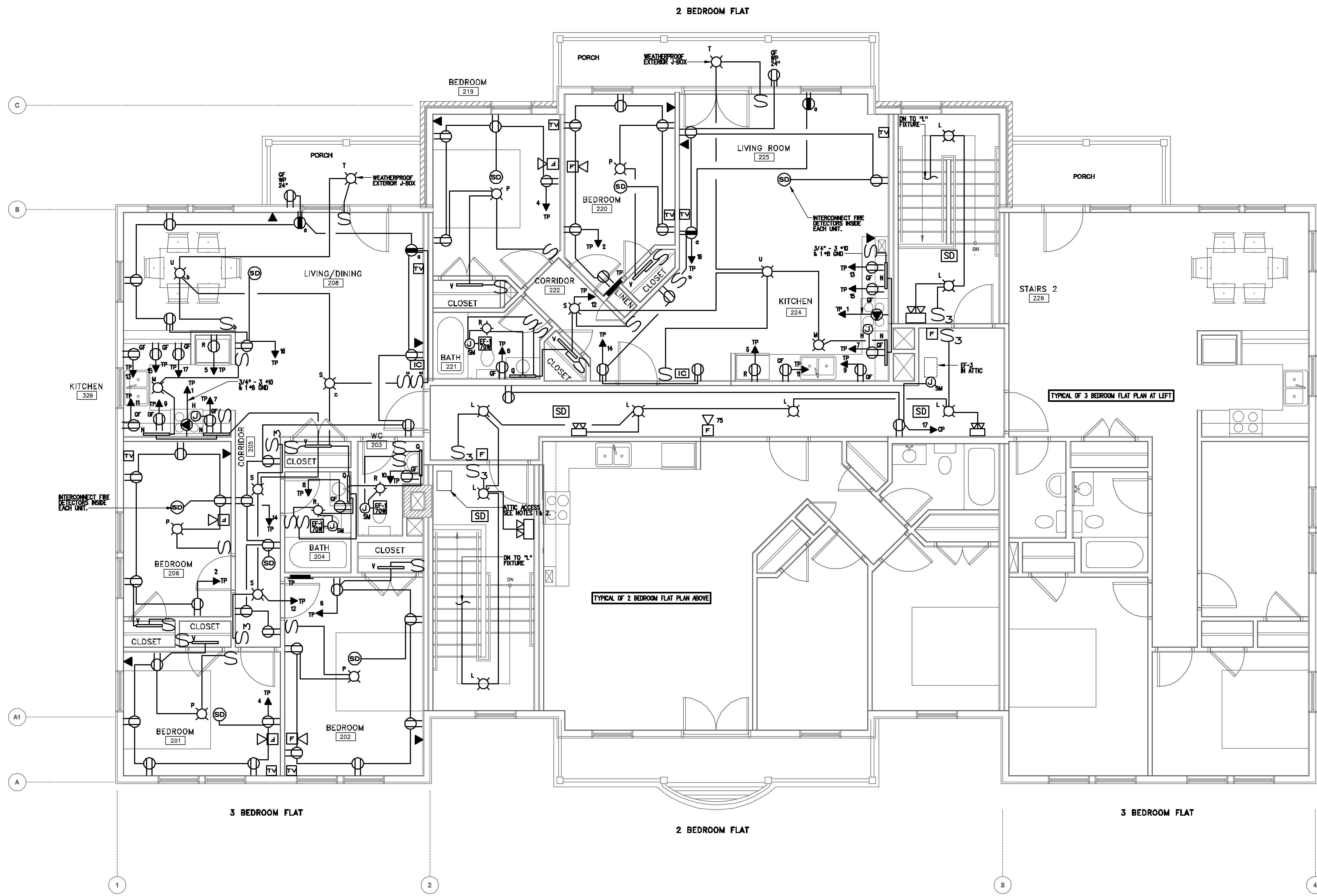
1 THIRD FLOOR ELECTRICAL PLAN BUILDING A 1/4" = 1'-0"
