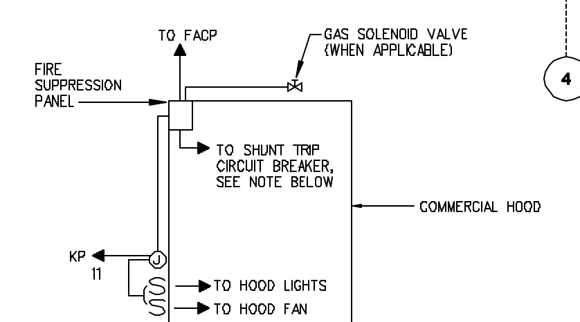
COMMERCIAL HOOD WIRING DETAIL NOT TO SCALE NOTE: OUTLETS UNDER HOOD SHALL BE SUPPLIED BY SHUNT TRIP CIRCUIT BREAKERS
