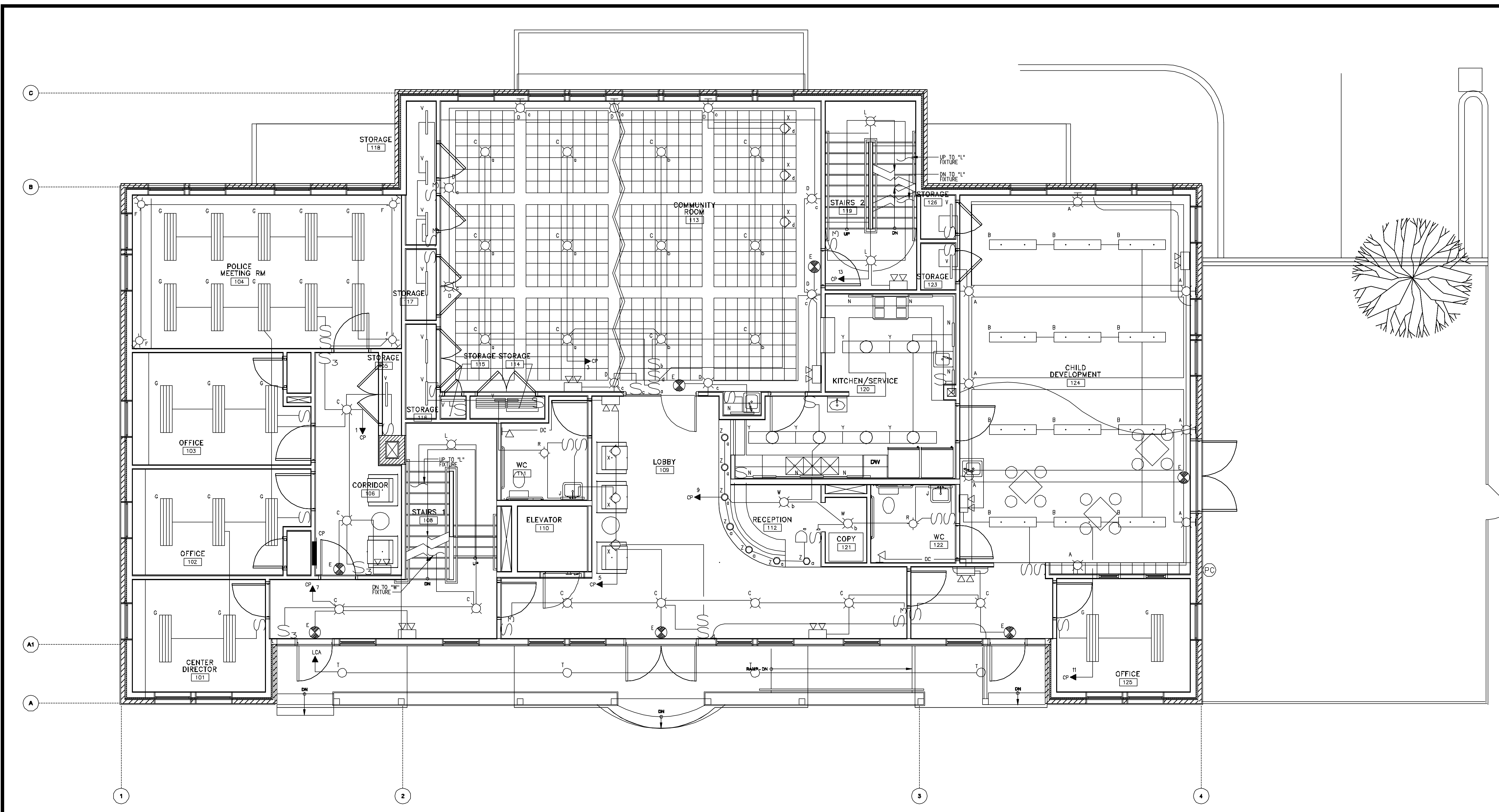
1 FIRST FLOOR LIGHTING PLAN BUILDING A 1/4" = 1'-0"
