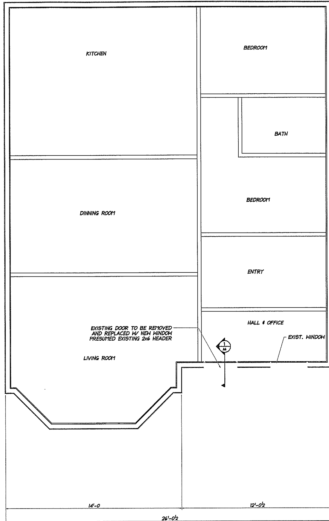
1 THIRD FLOOR A3 SCALE: 1/2" = 1'-0"
