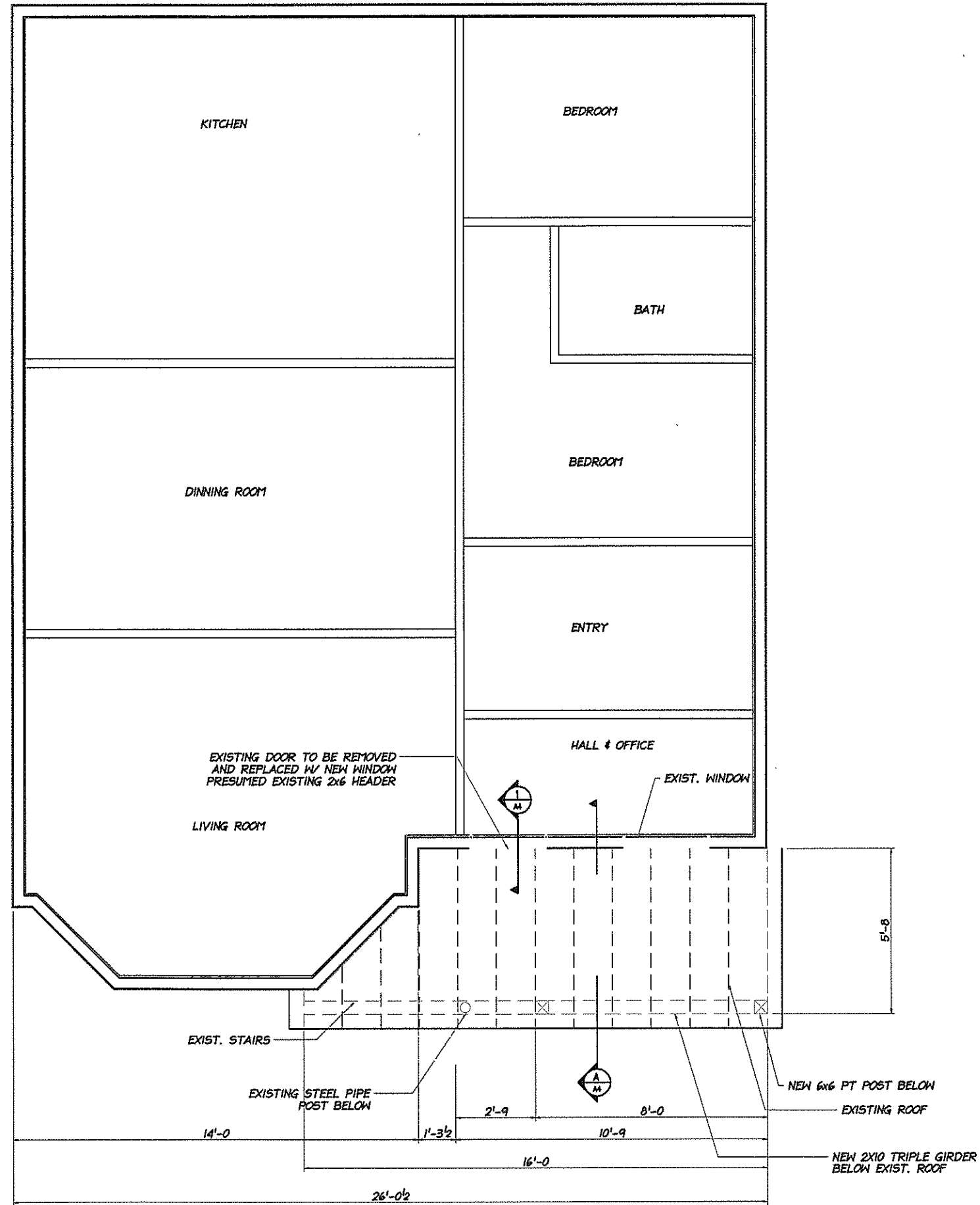
1 SECOND FLOOR A2 SCALE: 1/2"=1'-0"
