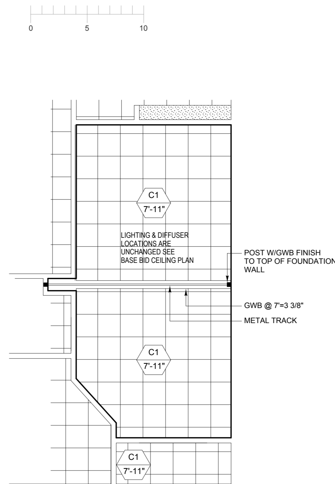
PART CEILING PLAN BY ALTERNATE #1 3/16" = 1'-0"
