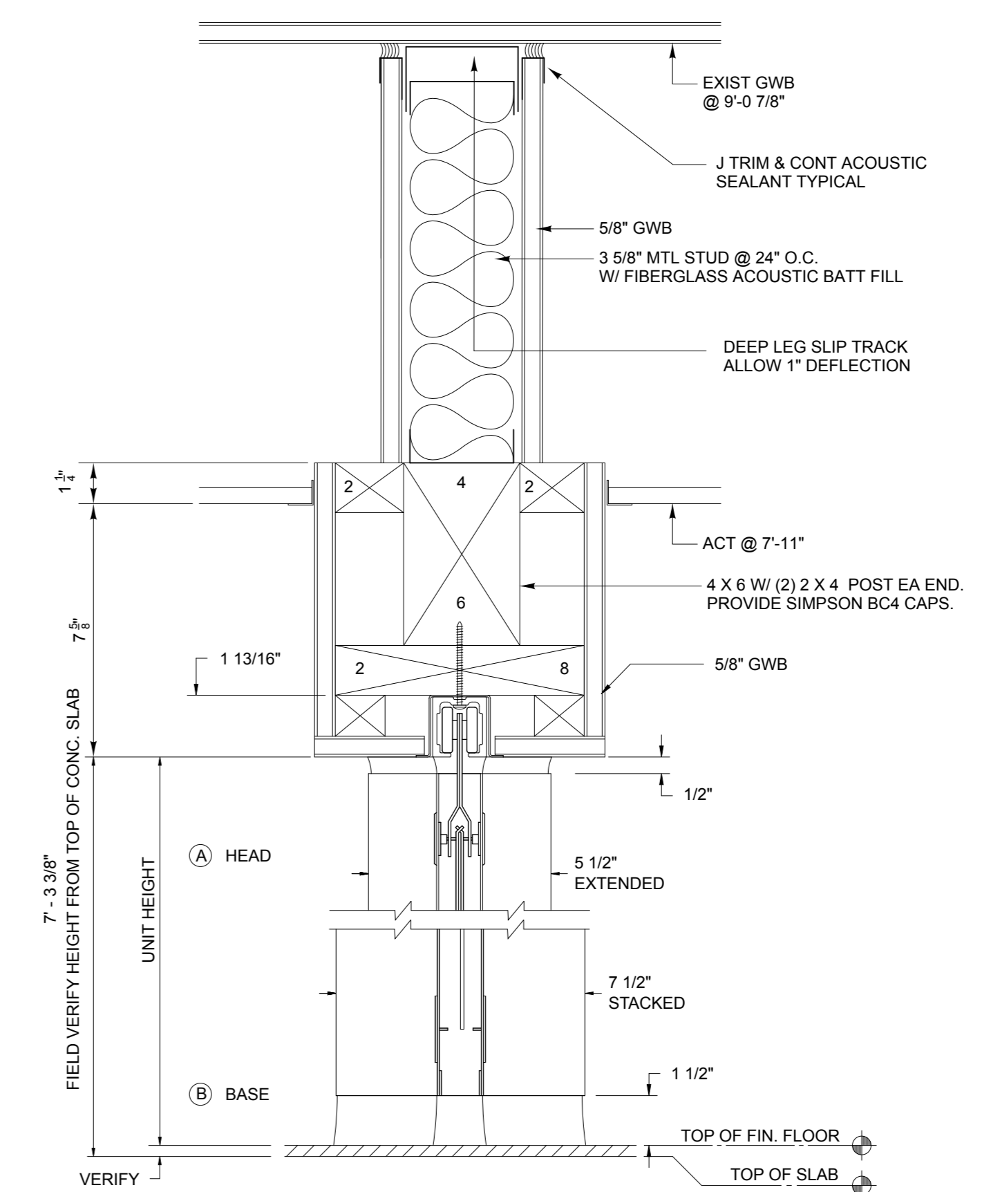
ACCORDION PARTITION SECTION - ALTERNATE #1 3" = 1'-0"
