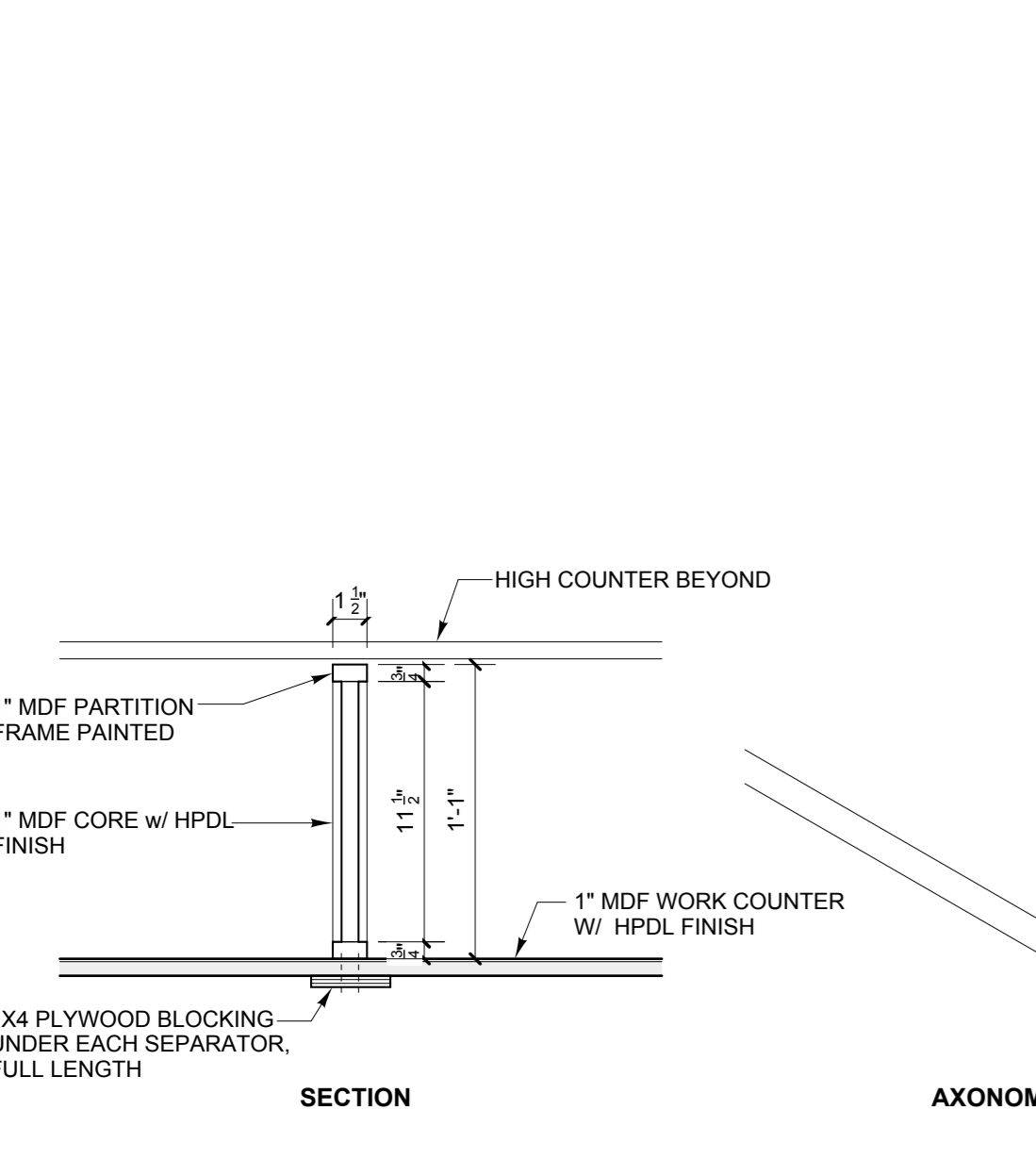
K DETAIL AT SEPARATOR SCALE: 1 1/2" = 1'-0"
