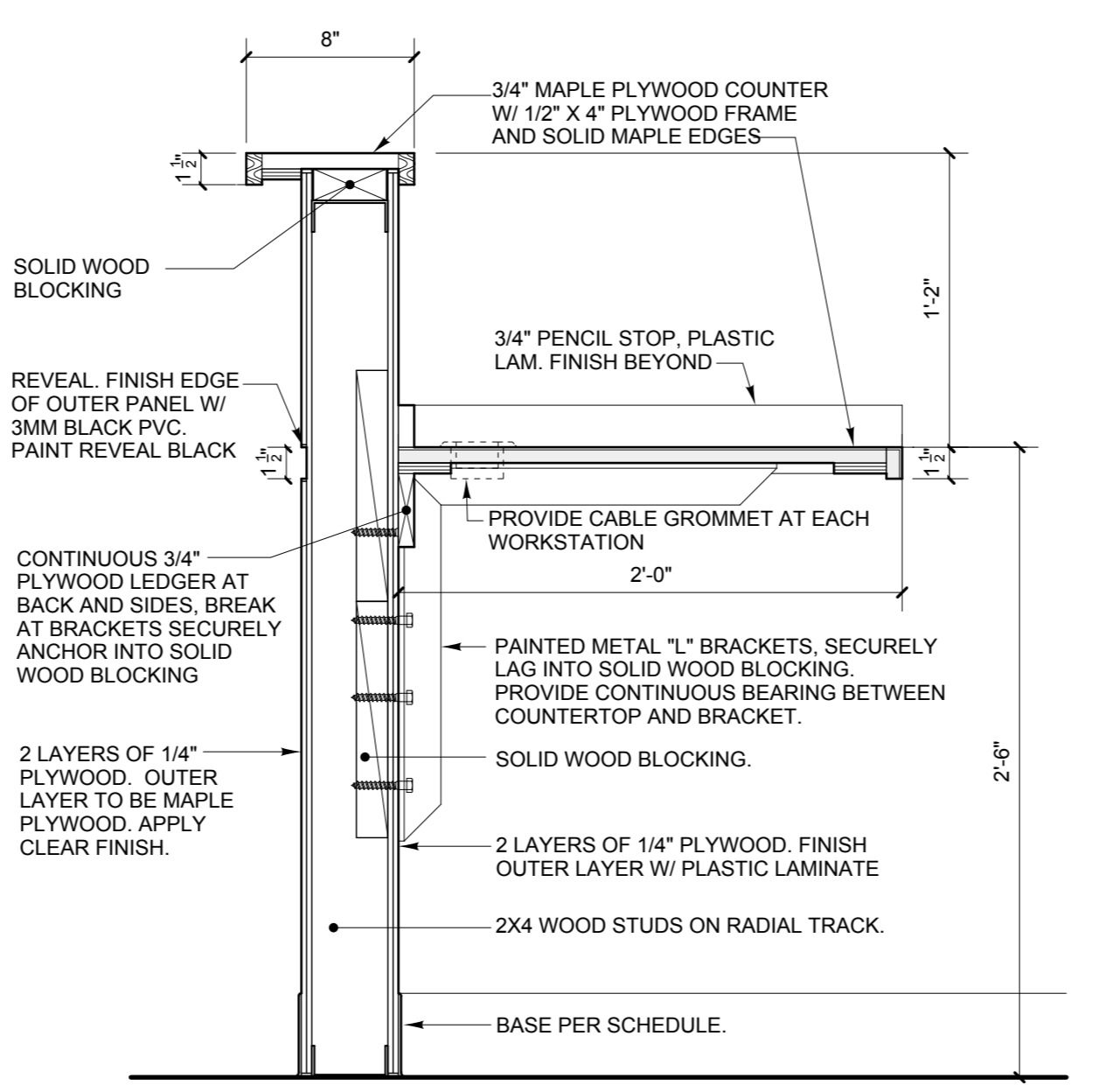
C SECTION DETAIL AT CHECK-IN / OUT 103 SCALE: 1 1/2" = 1'-0" SIMILAR AT REFER. COORD. 105
