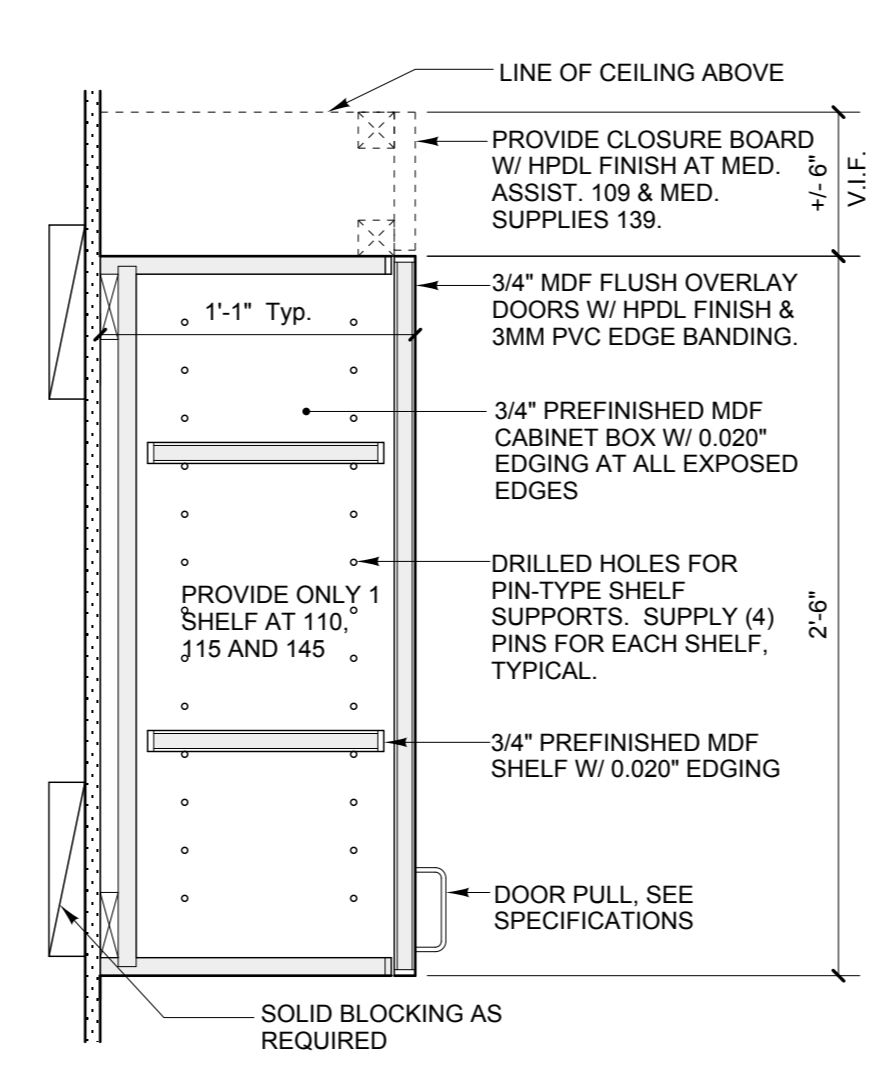
H UPPER CABINET DETAIL SCALE: 1 1/2" = 1'-0"
