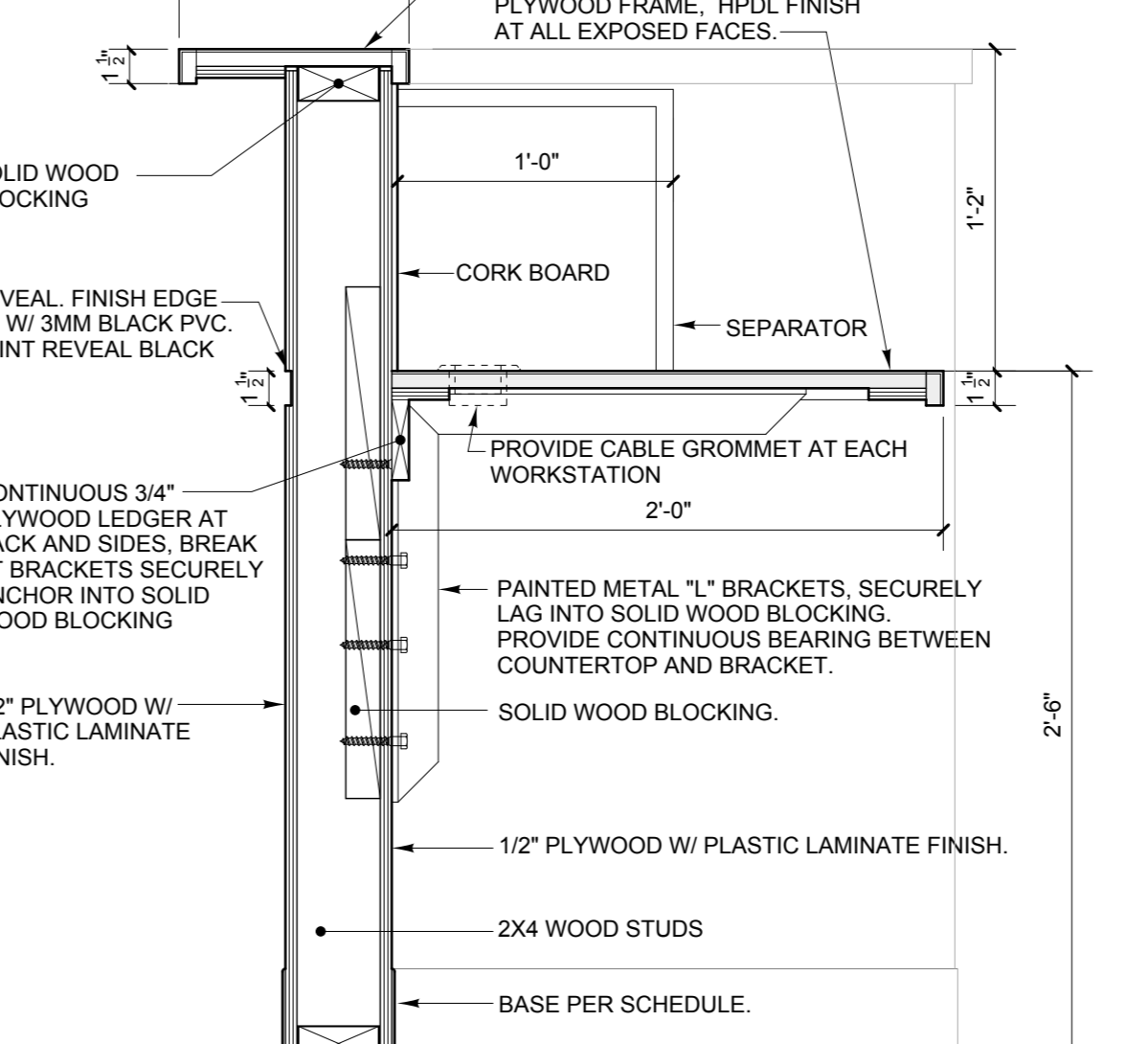
I SECTION DETAIL AT MED. ASSIST. 109 SCALE: 1 1/2" = 1'-0"
