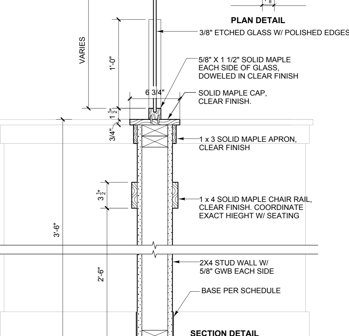
J KNEE WALL DETAIL SCALE: 1 1/2" = 1'-0"
