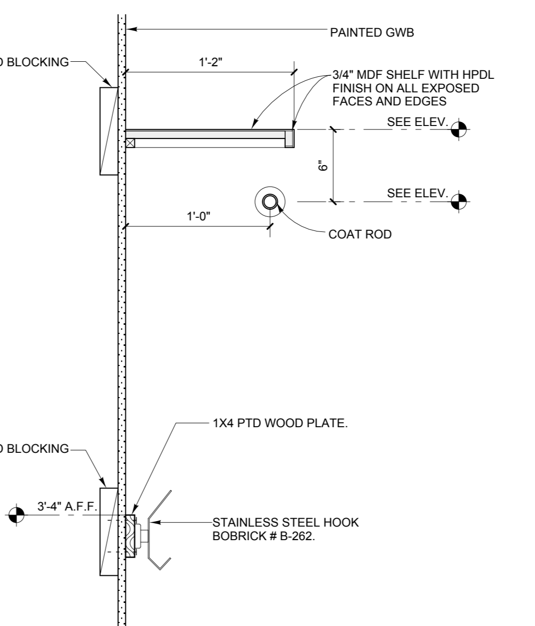
M TYPICAL COAT CLOSET DETAIL SCALE: 1 1/2" = 1'-0"
