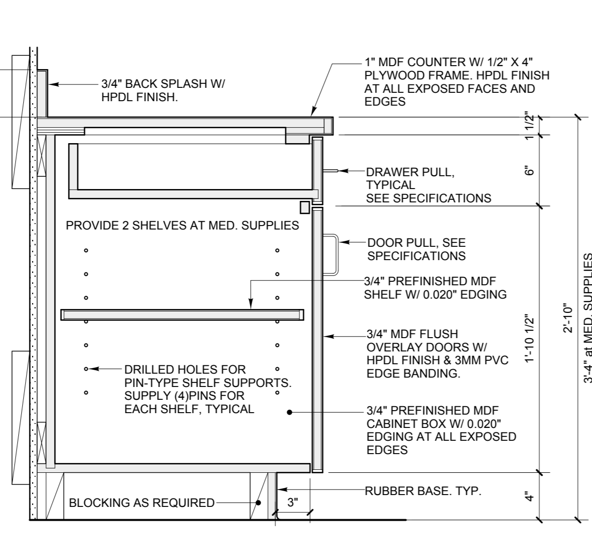
G BASE CABINET DETAIL AT BREAK ROOM SCALE: 1 1/2" = 1'-0"
