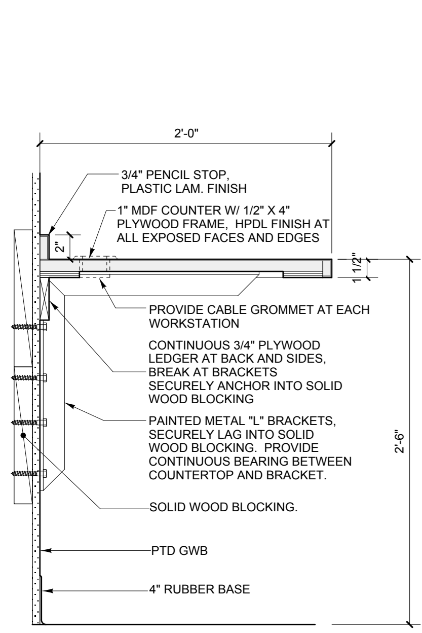
A COUNTER DETAIL W/ BRACKETS SCALE: 1 1/2" = 1'-0"
