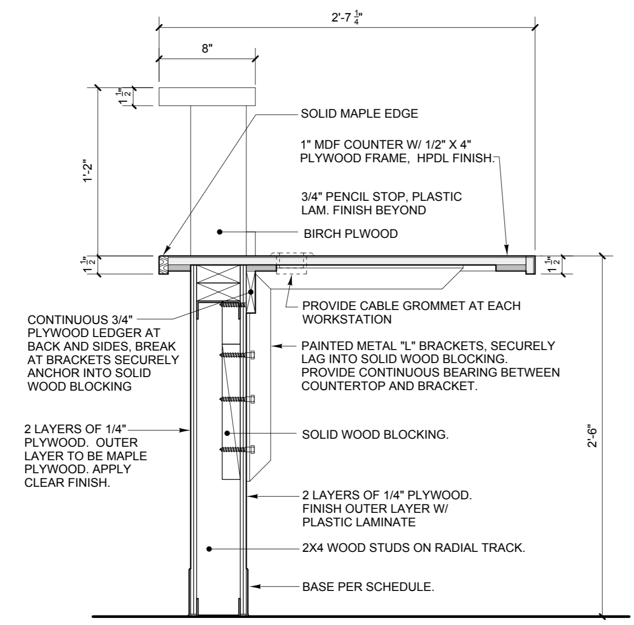
B SECTION DETAIL AT CHECK-IN / OUT 103 SCALE: 1 1/2" = 1'-0"
