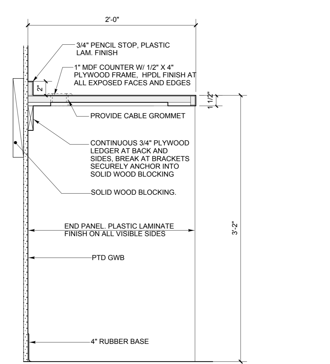
N PRINTER COUNTER DETAIL AT 107 SCALE: 1 1/2" = 1'-0"
