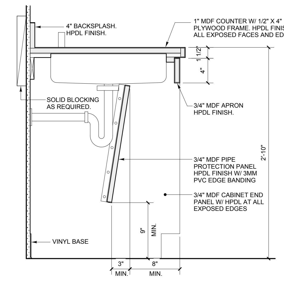
F SECTION DETAIL AT SINK SCALE: 1 1/2" = 1'-0"
